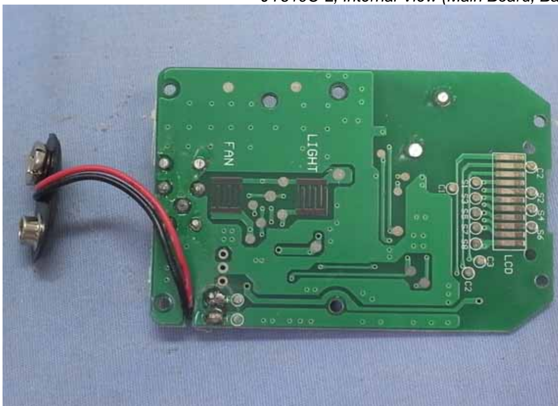
Photo 12 JY610C-L, Internal View (Main Board, Back View)
