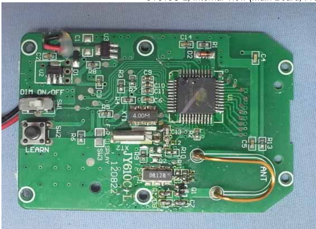
Photo 11 JY610C-L, Internal View (Main Board, Front View)
