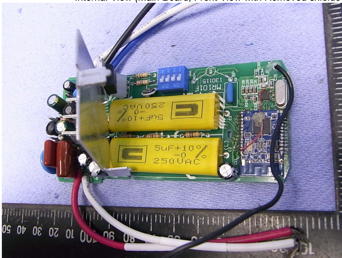
Photo 5 Internal View (Main Board, Front View with Removed shielded Cover)
