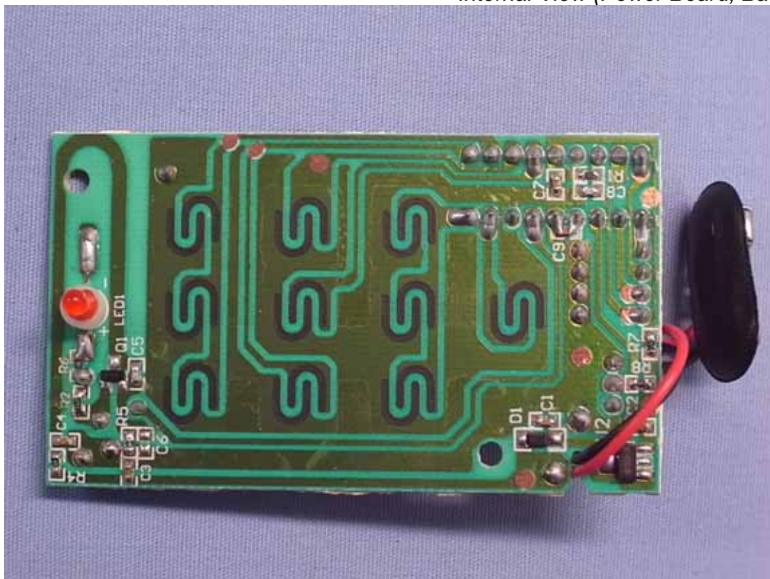
Photo 5 Internal View (Power Board, Back View)
