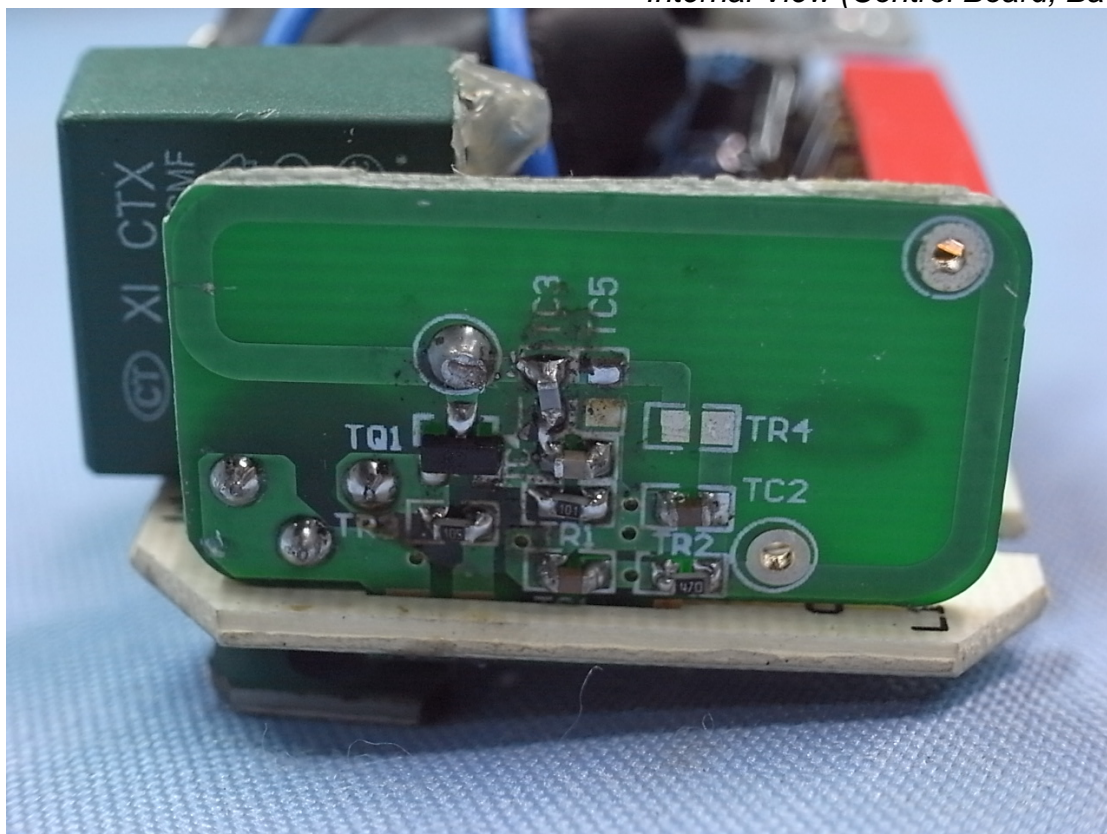
Photo 8 Internal View (Control Board, Back View)
