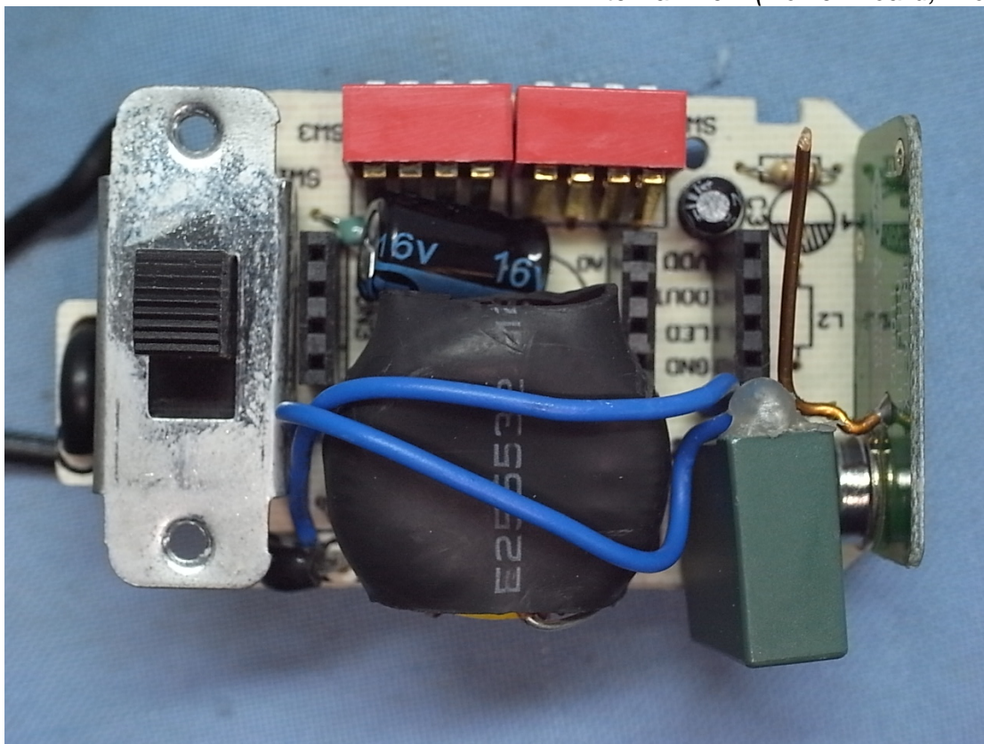
Photo 5 Internal View (Power Board, Front View)
