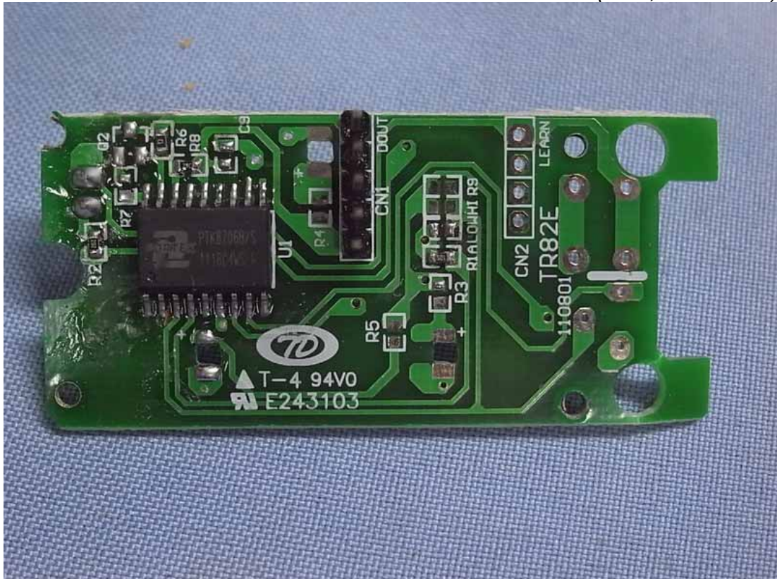
Photo 7 Internal View (PCB, Front View)
