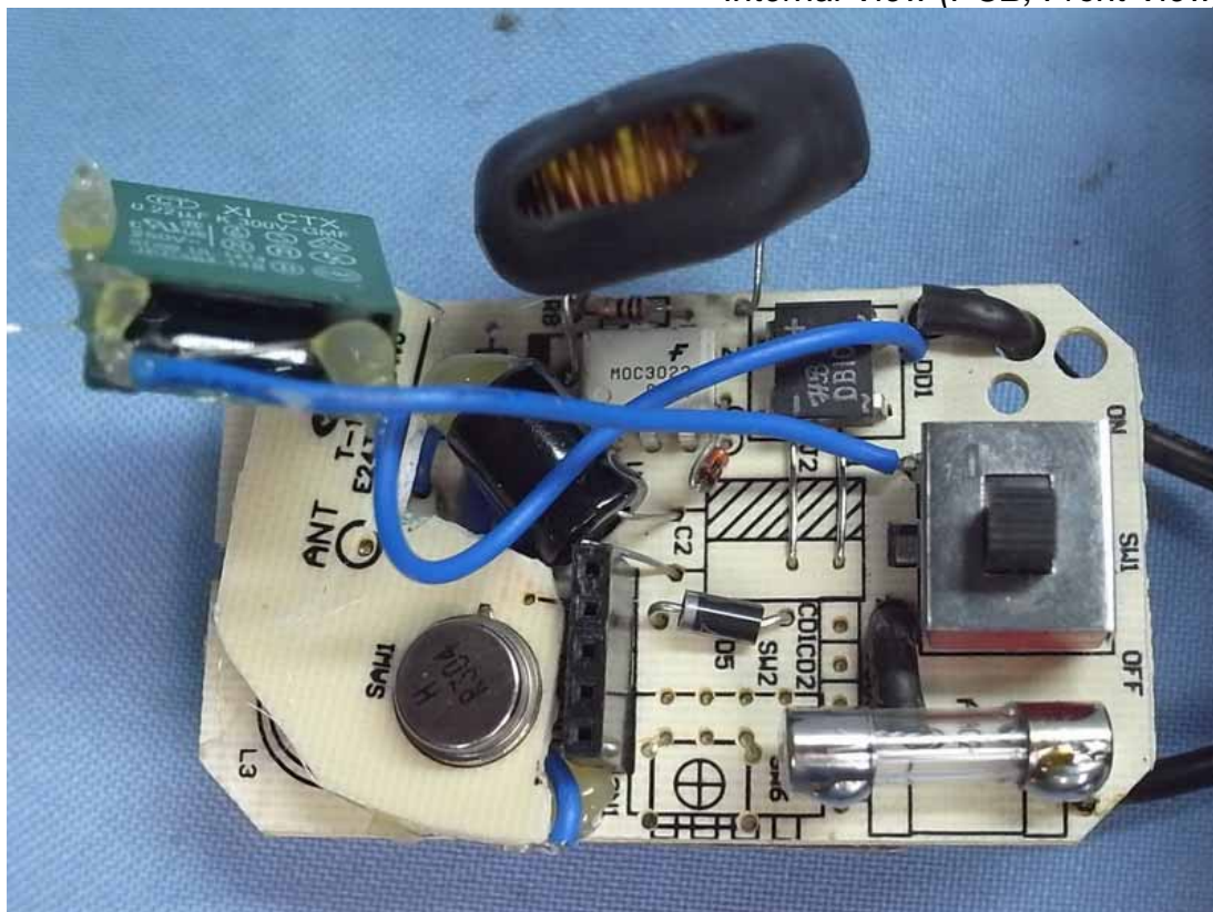
Photo 5 Internal View (PCB, Front View)
