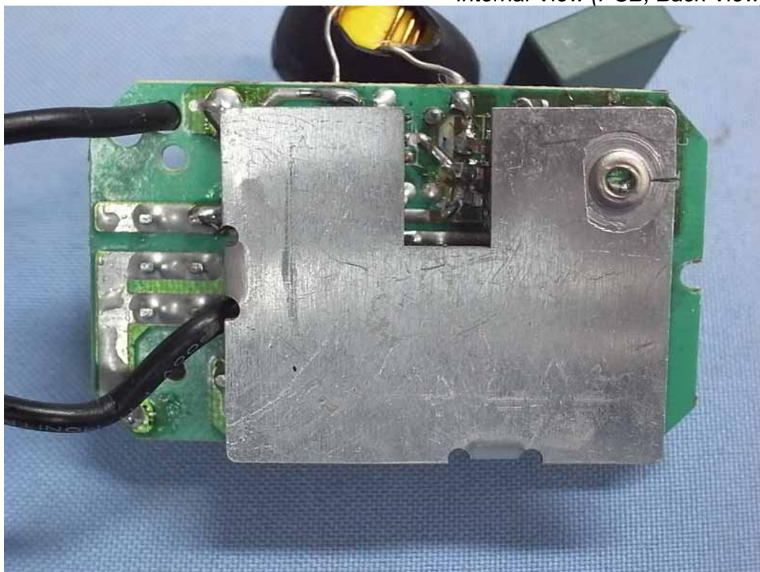
Photo 6 Internal View (PCB, Back View)
