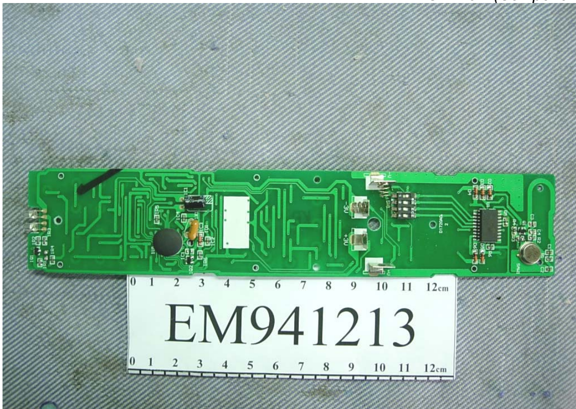
Photo 4 PCB View (Component Side)
