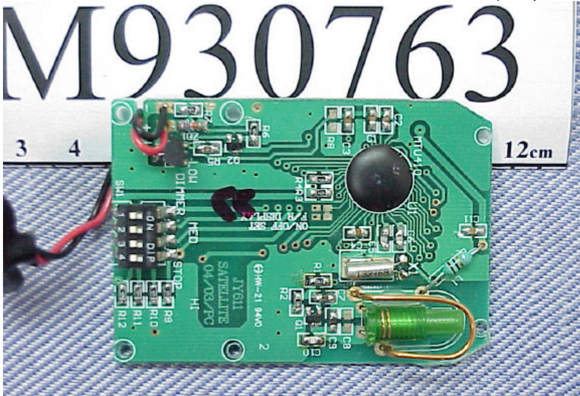
Photo 5 PCB View (Component Side)
