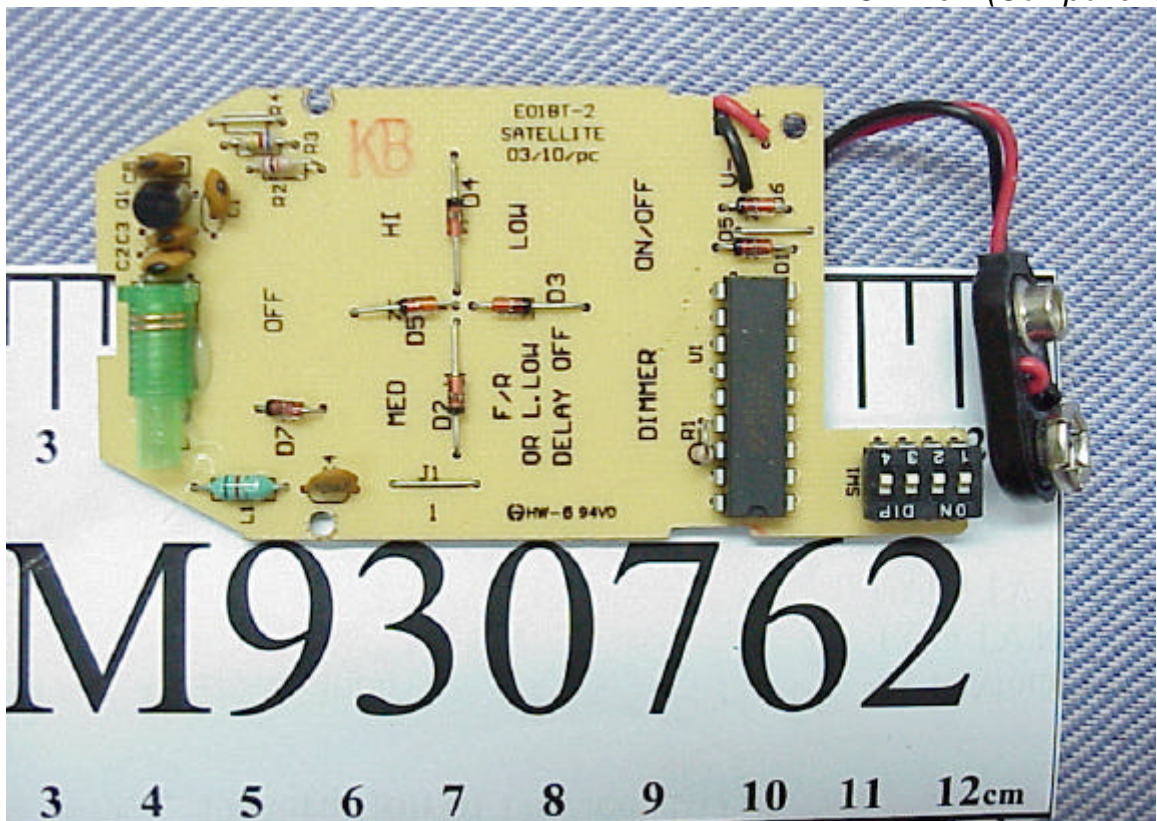
Photo 5 PCB View (Component Side)
