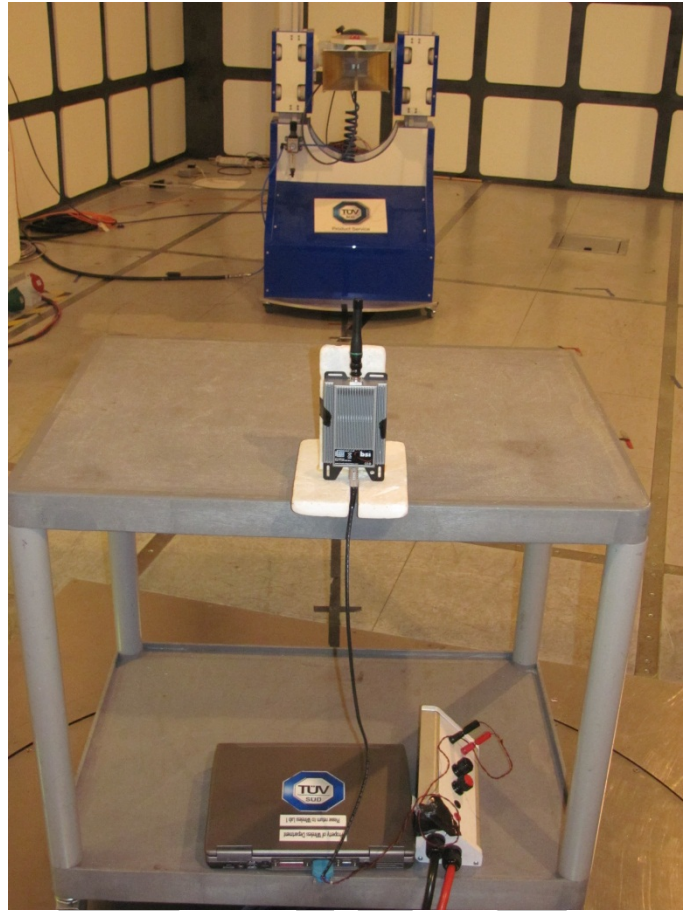
FCC CFR 47 Part 15B - Radiated Emissions 1 GHz to 3 GHz
