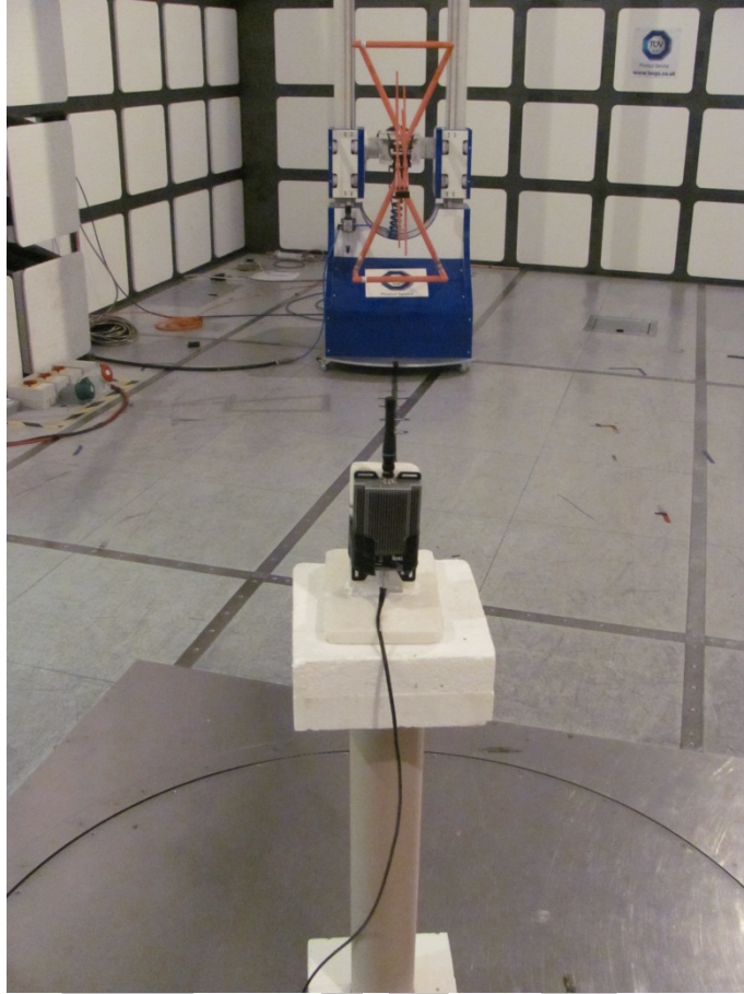
FCC CFR 47 Part 90 - Radiated Emissions 30 MHz to 1 GHz (Upright)
