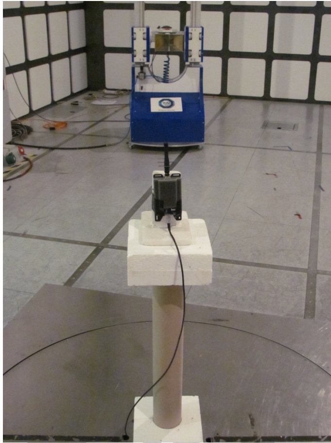
FCC CFR 47 Part 90 - Radiated Emissions 1 GHz to 5 GHz (Upright)
