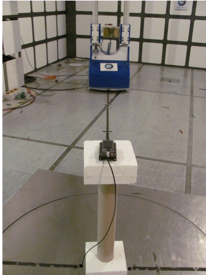
FCC CFR 47 Part 90 - Radiated Emissions 1 GHz to 5 GHz (On Back)
