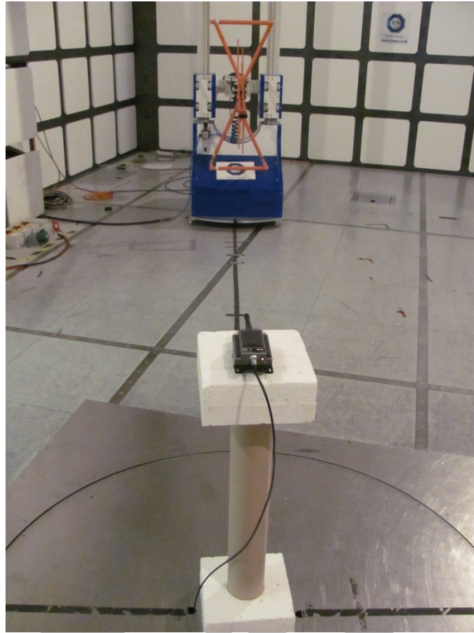
FCC CFR 47 Part 90 - Radiated Emissions 30 MHz to 1 GHz (On Back)
