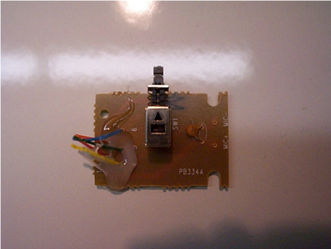
PC Board-Component Side – Hand TX
