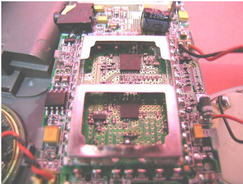
Handset Oscillator PCB comp side (View 4)
