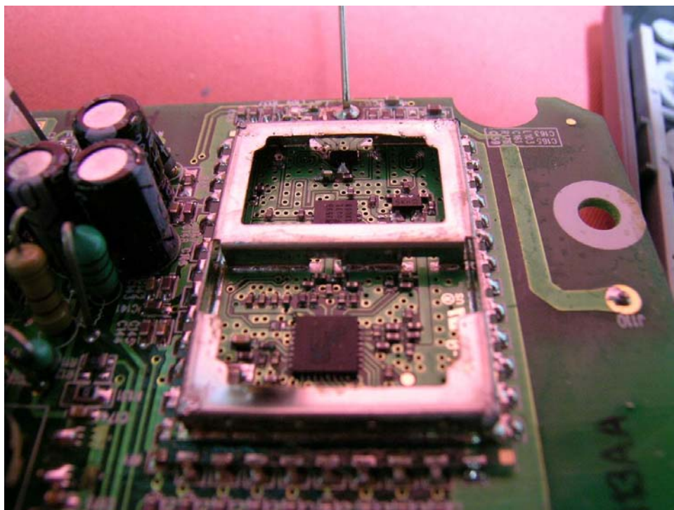
Base Oscillator PCB comp side (View 3)
