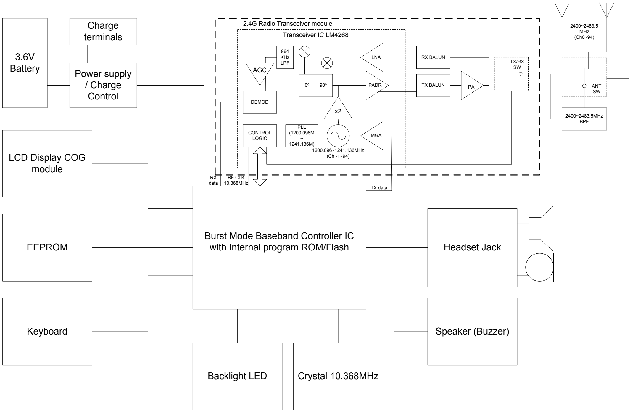
TW338/339/339H Handset Block Diagram
