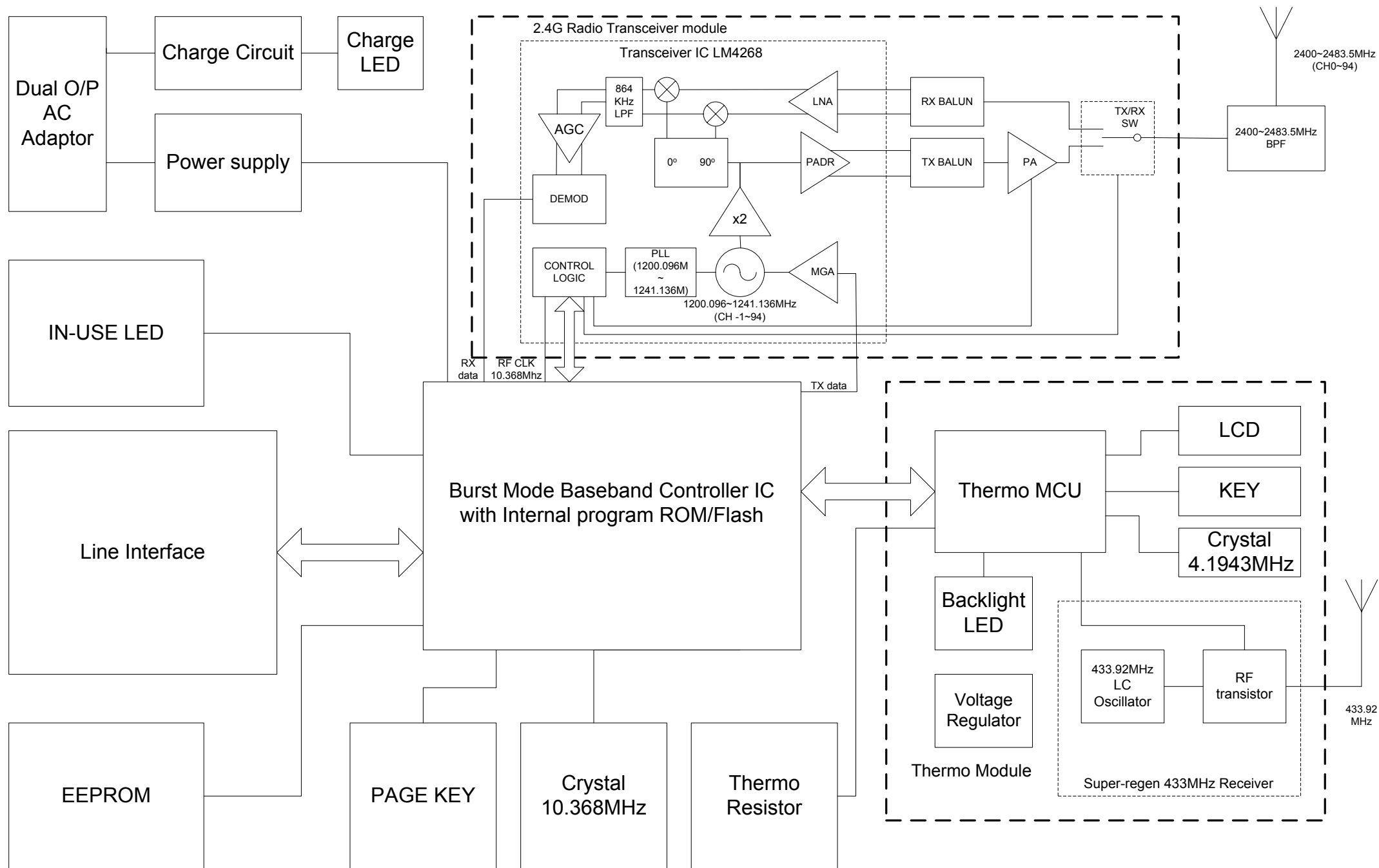
TW338/339/339H Base Unit Block Diagram
