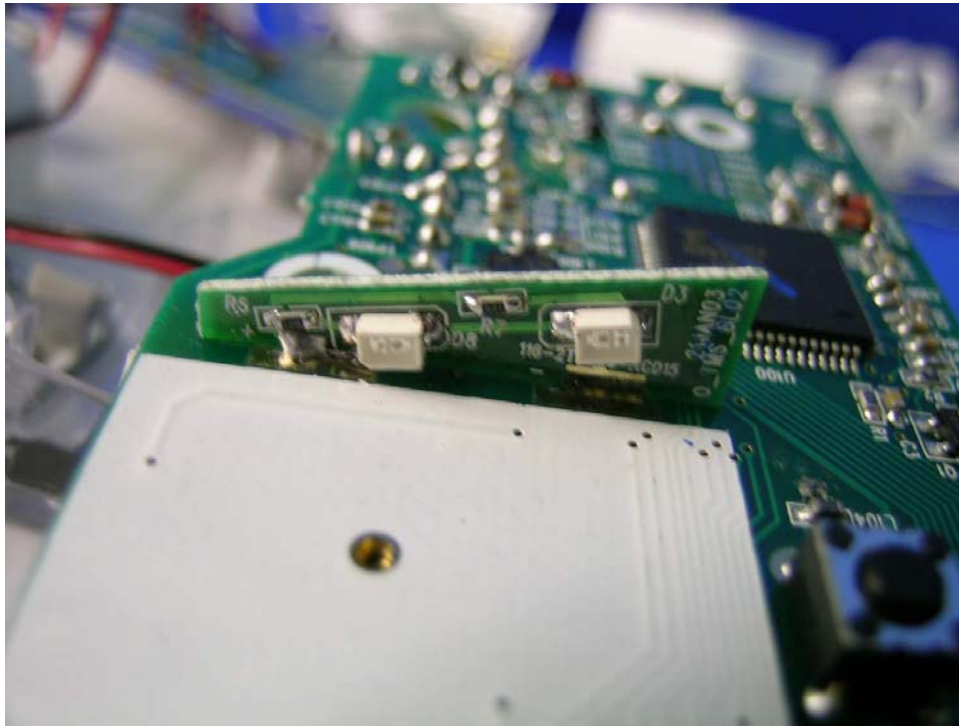
Base Remote Thermo Sensor PCB solder side (View 3)
