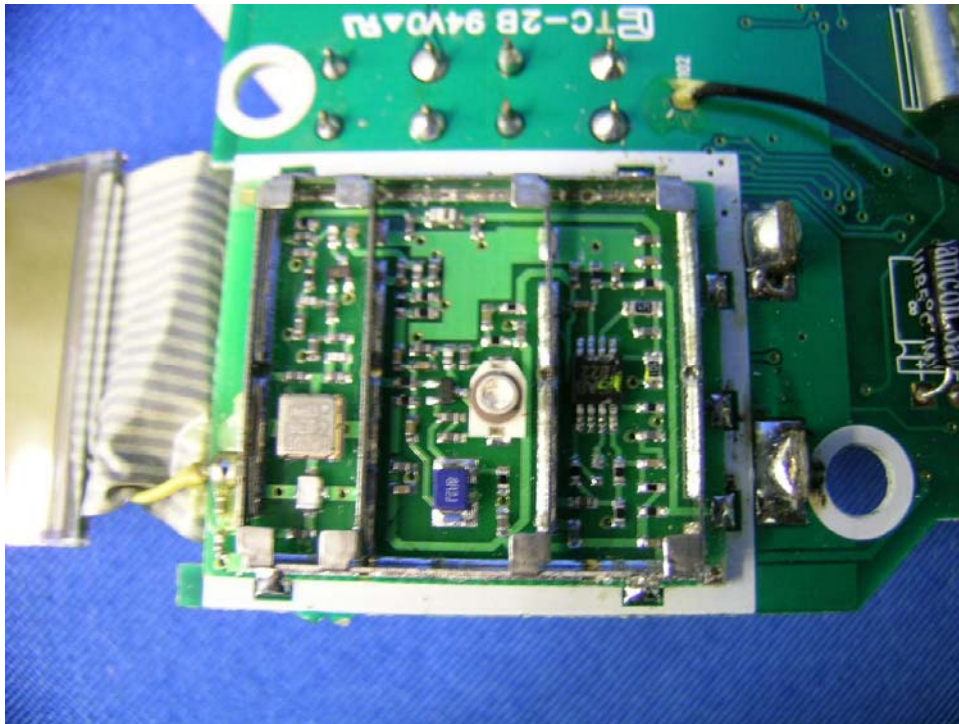
Base Remote Thermo Sensor Oscillator PCB comp side
