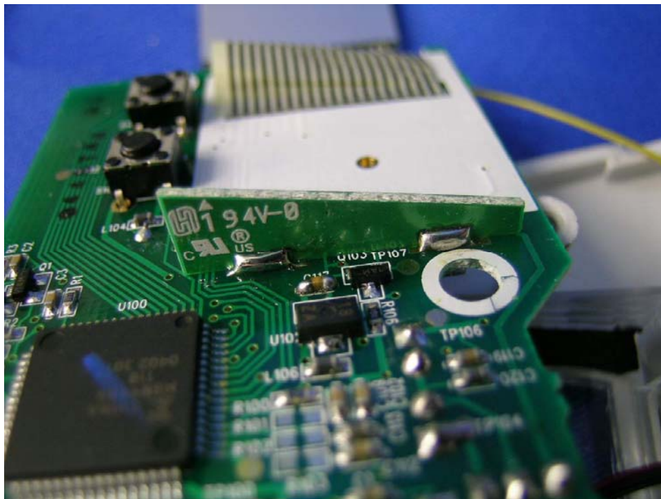
Base Remote Thermo Sensor PCB solder side (View 2)
