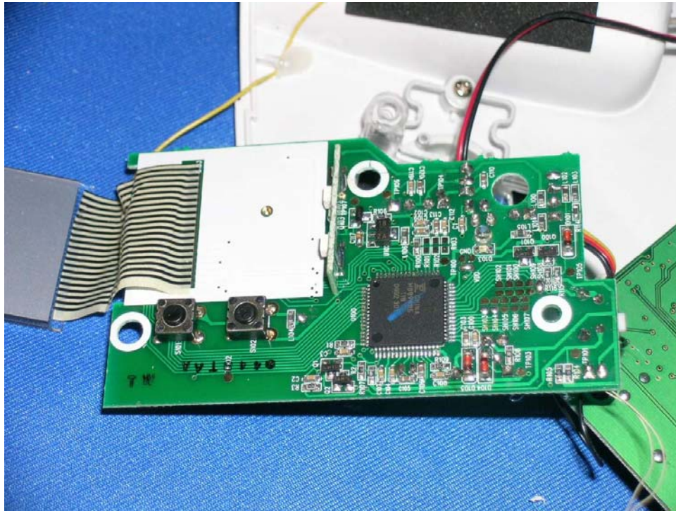
Base Remote Thermo Sensor PCB solder side (View 1)
