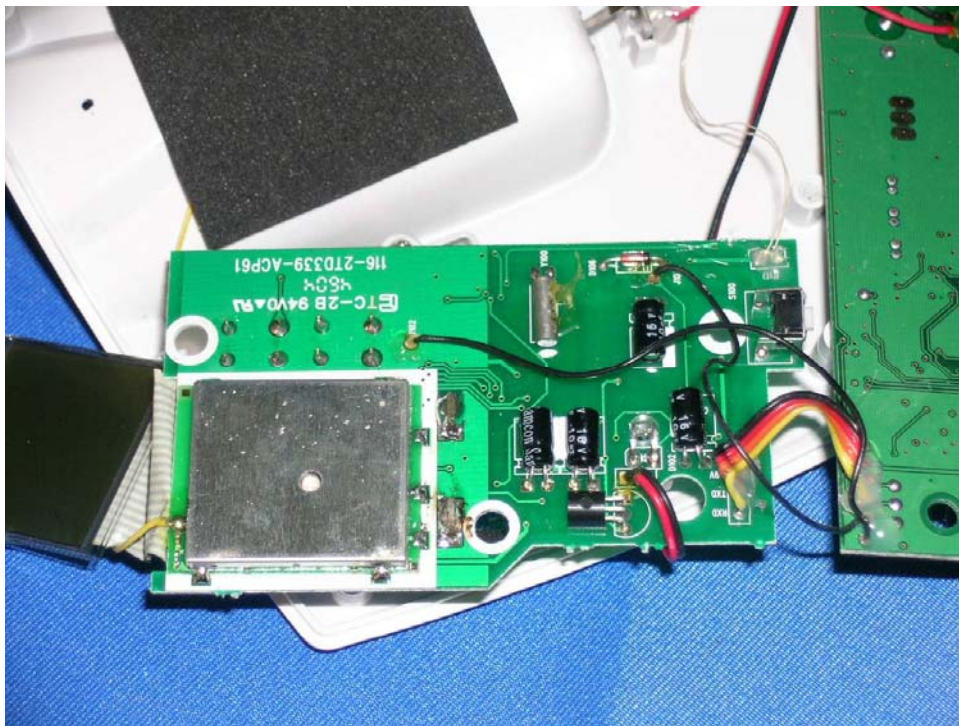
Base Remote Thermo Sensor PCB comp side
