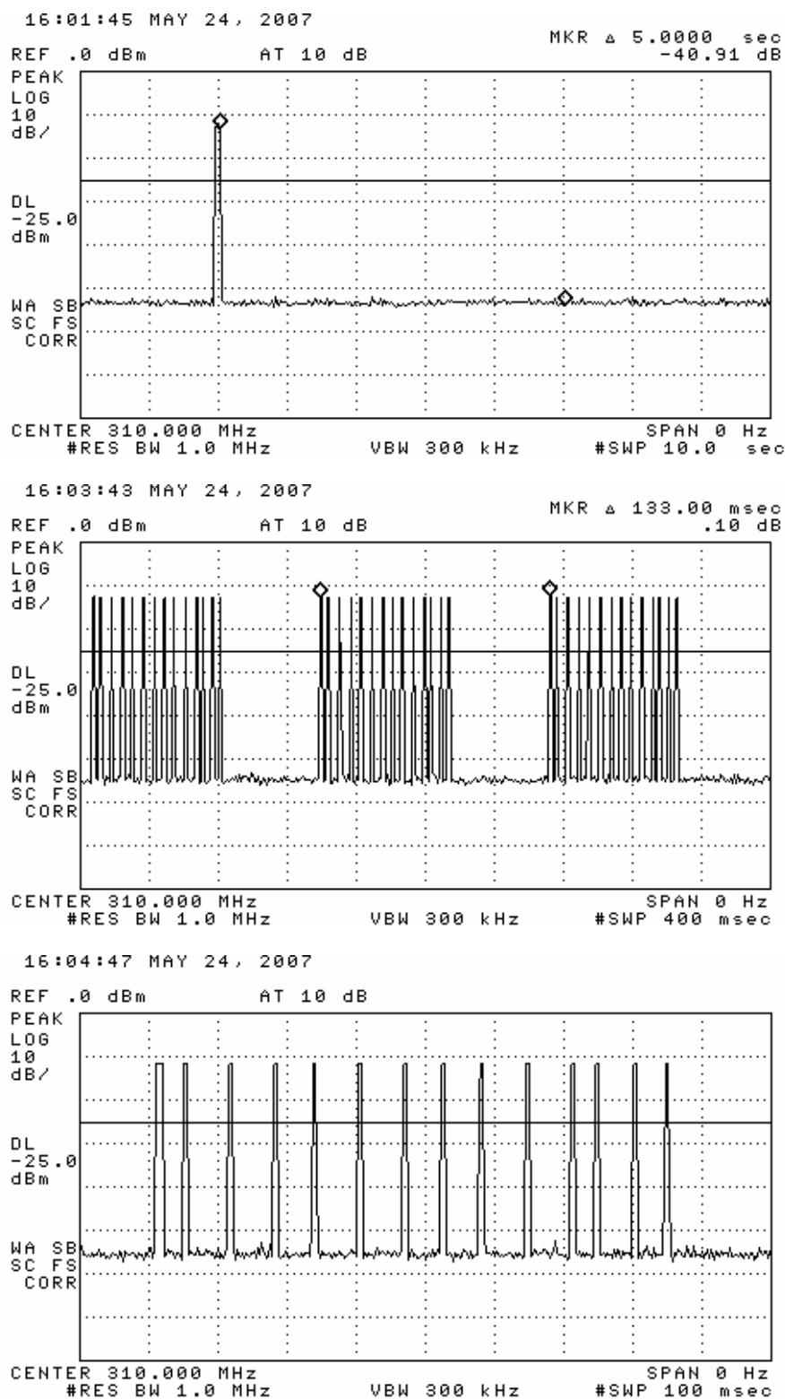
Figure 6.1(a). Transmissions modulation characteristics: (top) single activation, (center) repeated transmission , (bottom) expanded word.
