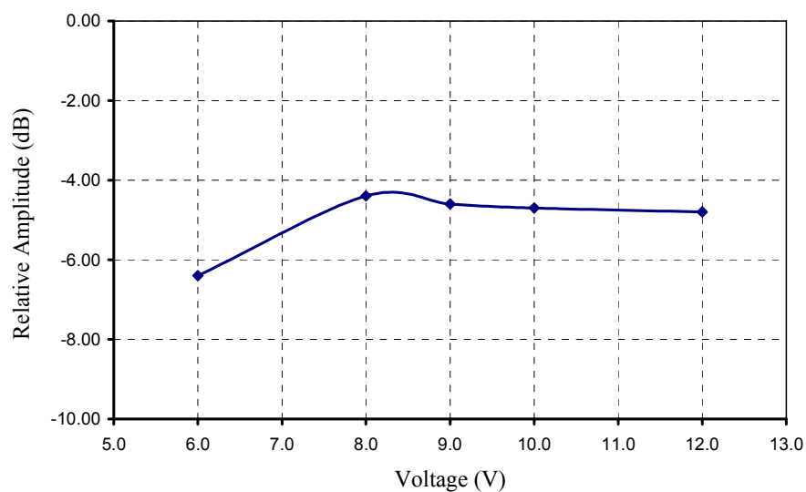
Figure 6.5. Relative emission at 310 MHz vs. supply voltage (pulsed emission).
