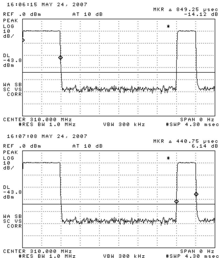
Figure 6.1(b). Transmissions modulation characteristics: (top) wake pulse, (bottom) coding pulse width.
