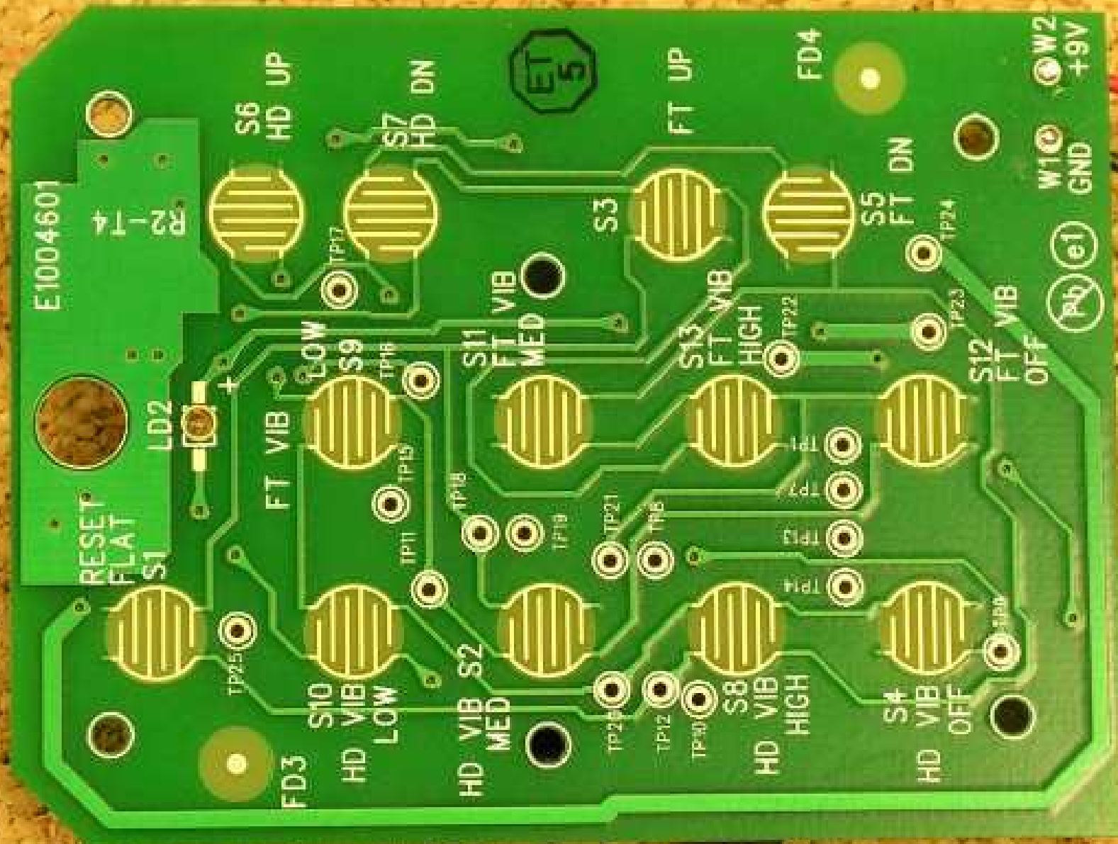
PCB (top)
