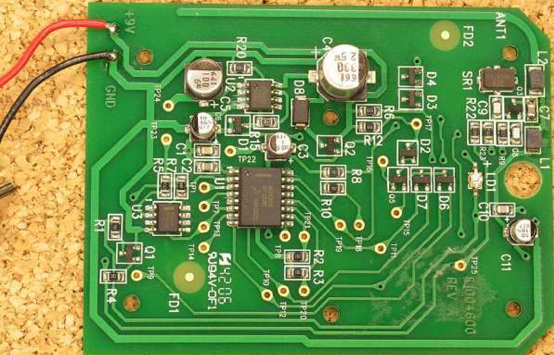
PCB (bottom)
