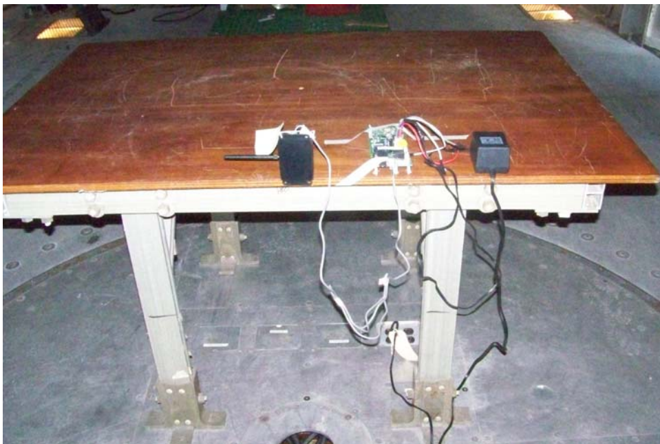
Radiated Emissions, Rear View, Z-Axis Setup
