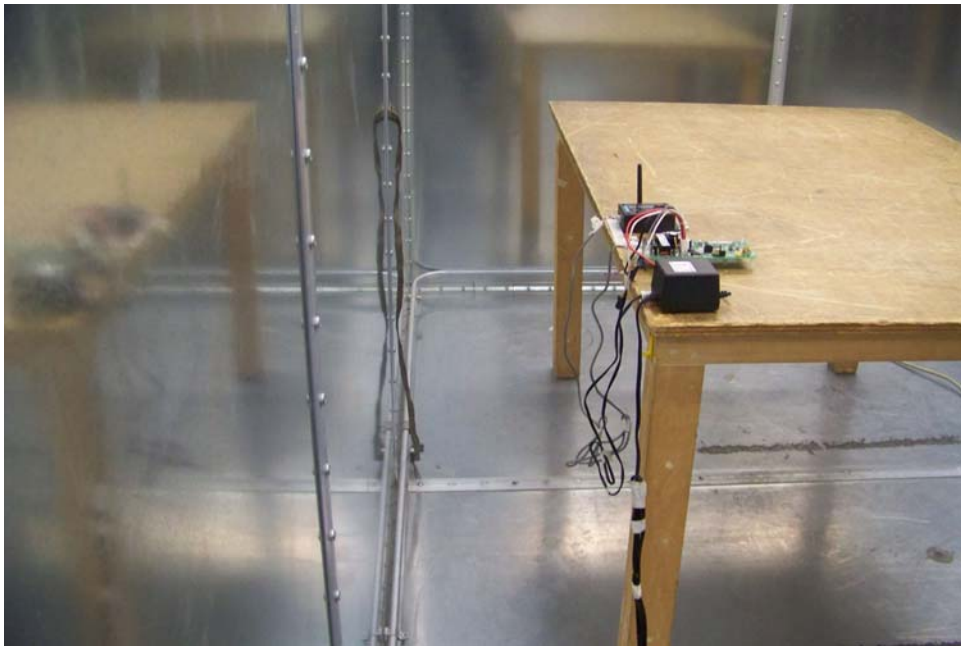
Conducted Emissions, Cable Layout
