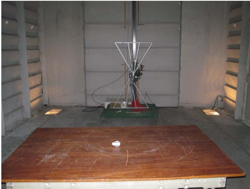
Transmitter, Biconilog Antenna, Vertical Polarity, Test Distance
