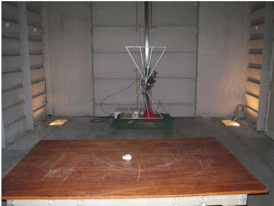
Receiver, Biconilog Antenna, Vertical Polarity, Test Distance
