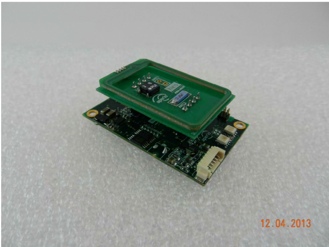
Antenna board mounted on main board
