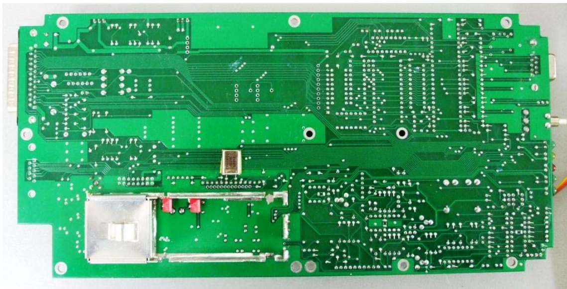
RX Main PCB
