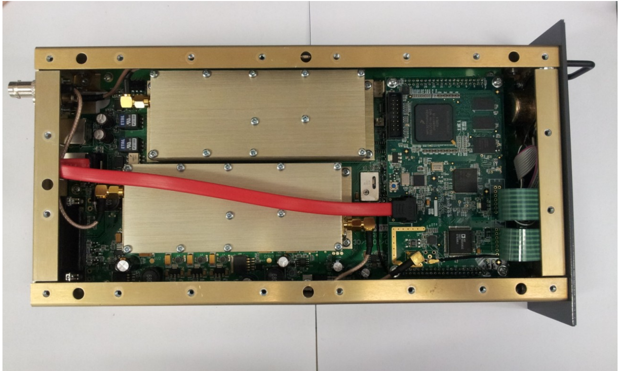
FULL ASSEMBLED ECLIPSE 2 BASE STATION – TOP VIEW
