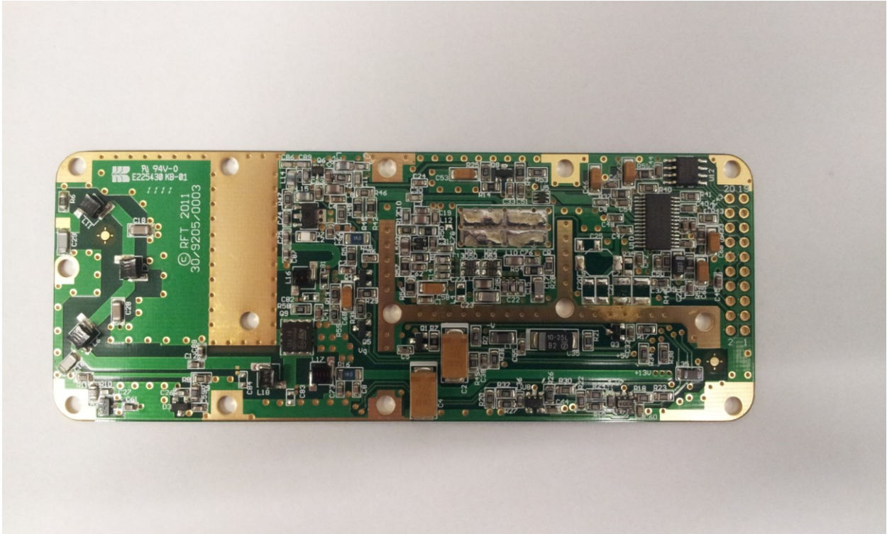
TX TOP VIEW
