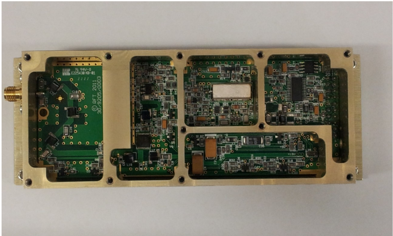
TX TOP VIEW WITH SHIELDS
