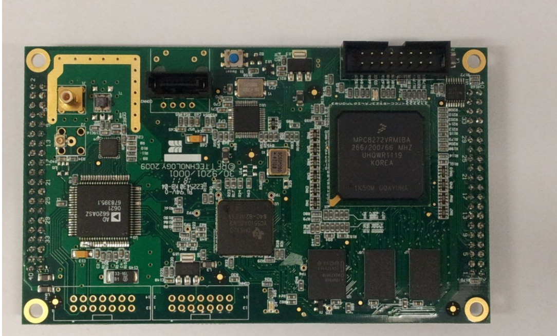
CONTROLLER BOARD – TOP VIEW
