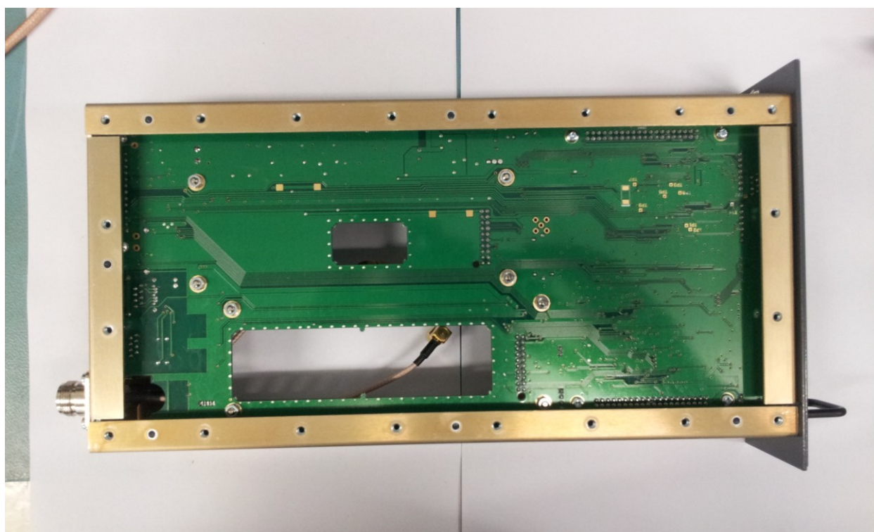
MAIN BOARD – BOTTOM VIEW – WITH SHIELD
