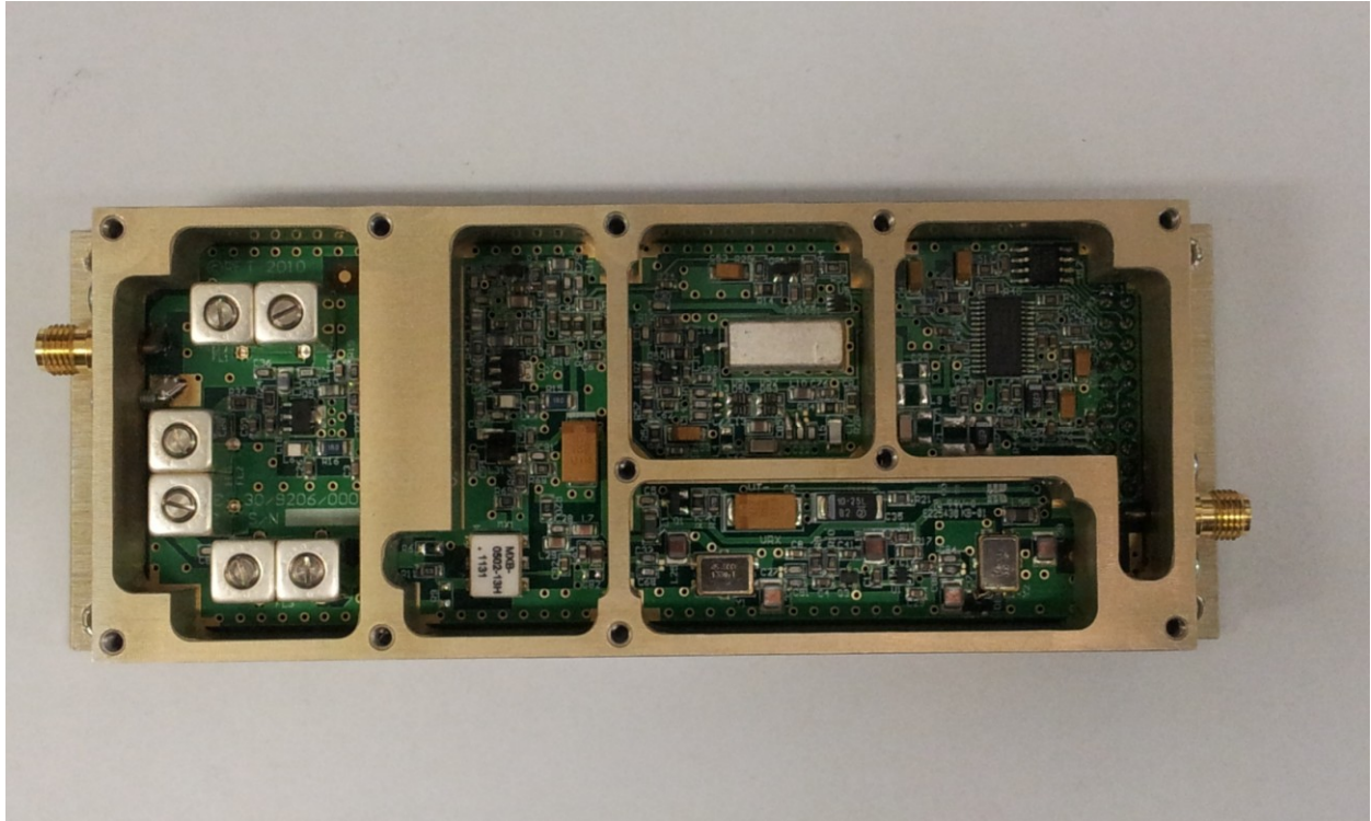
RX TOP VIEW WITH SHIELDS
