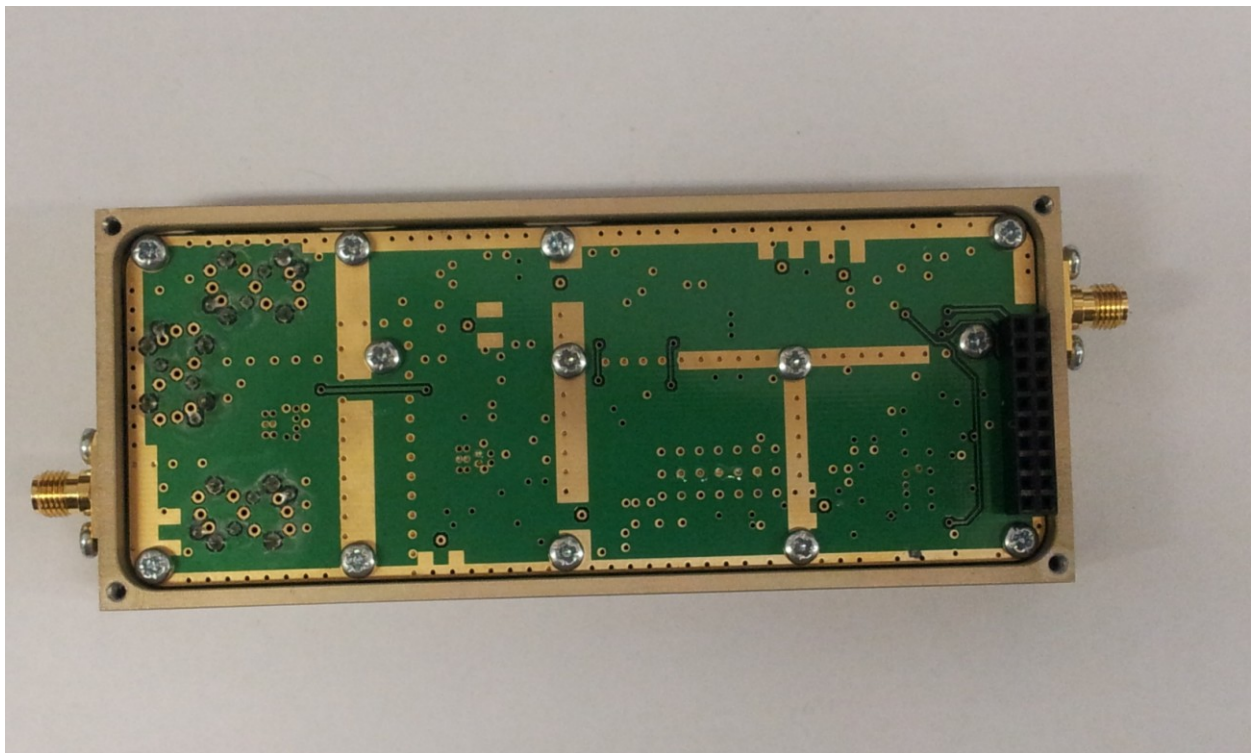
RX BOTTOM VIEW WITH SHIELDS
