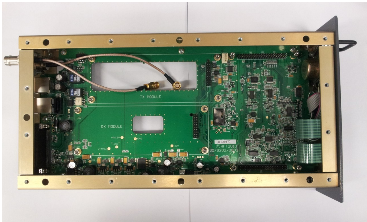
MAIN BOARD – TOP VIEW – WITH SHIELD
