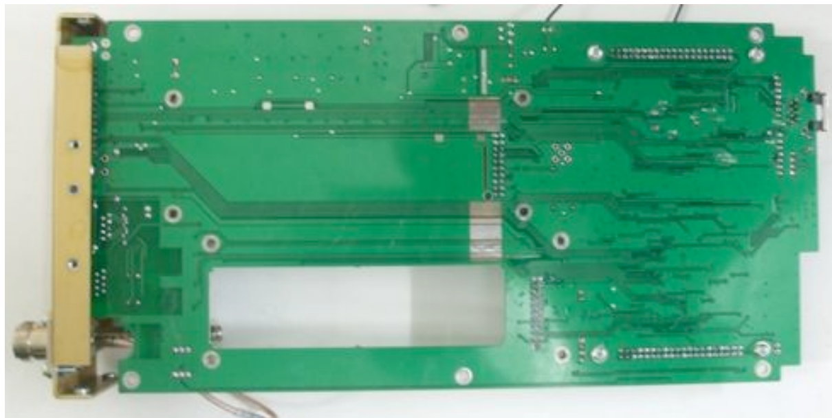
Main PCB
