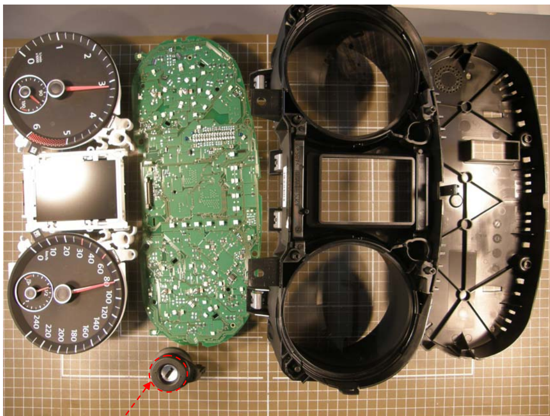
Loop antenna inside the plastic housing of the ignition lock Antenna area: 0.00071 \text{ m}^2
