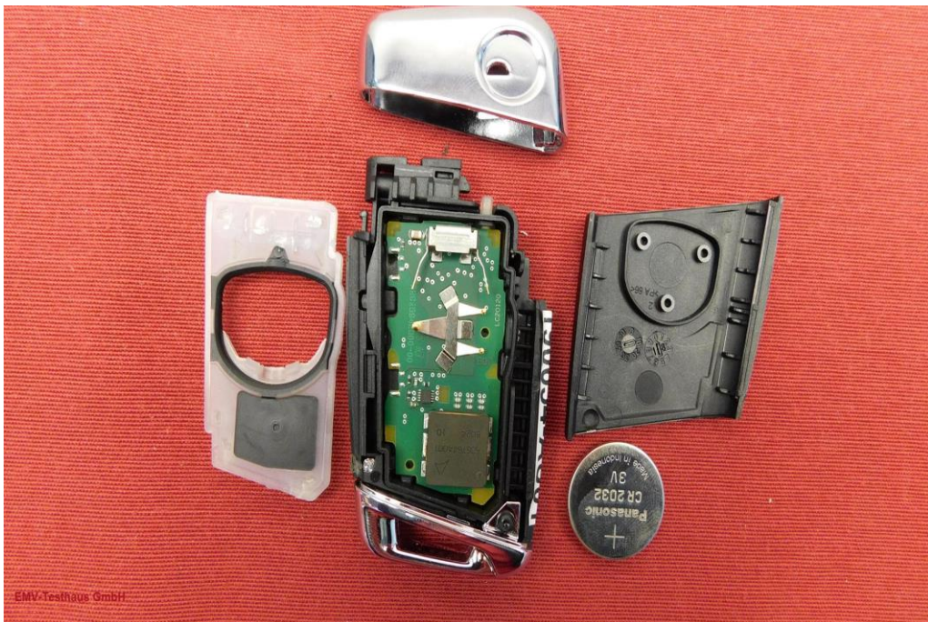
Picture 2: Opened FS14T, version FS14T without battery (top view)
