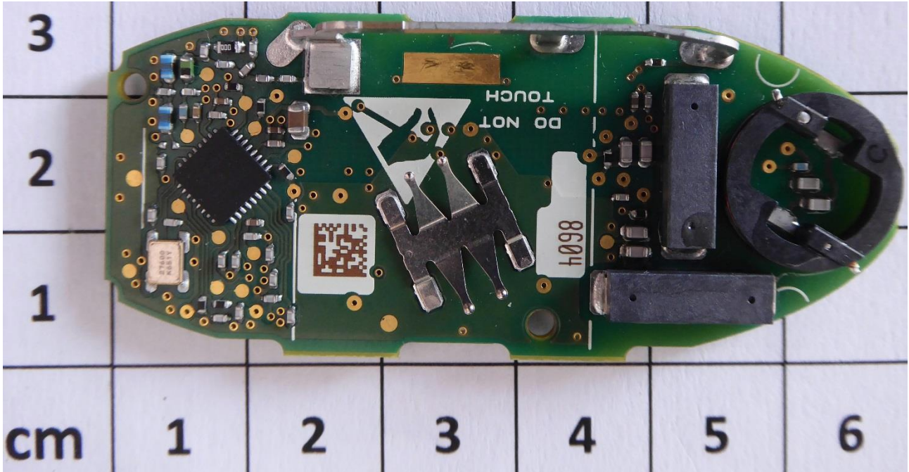
PCB front
