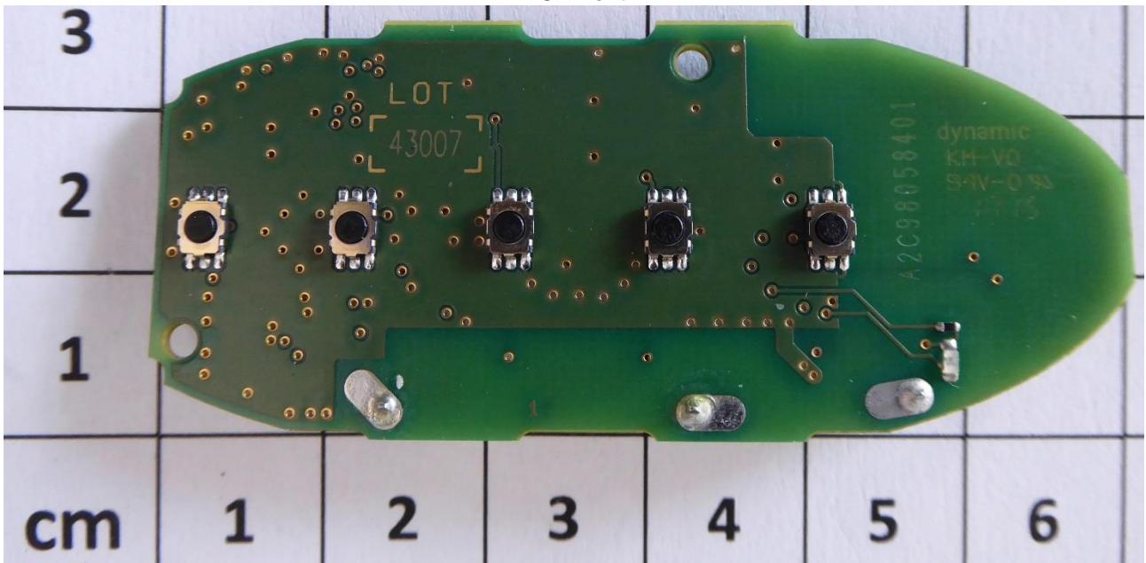
PCB front
