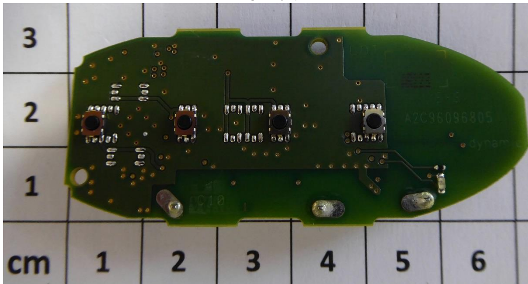
PCB front
