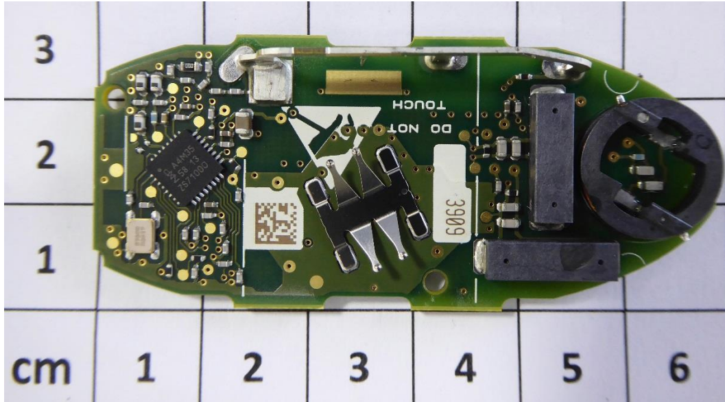
PCB front
