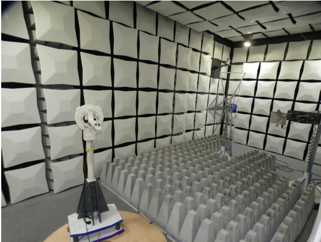
Photo 3: Test setup for radiated measurements (1 GHz – 26 GHz)
