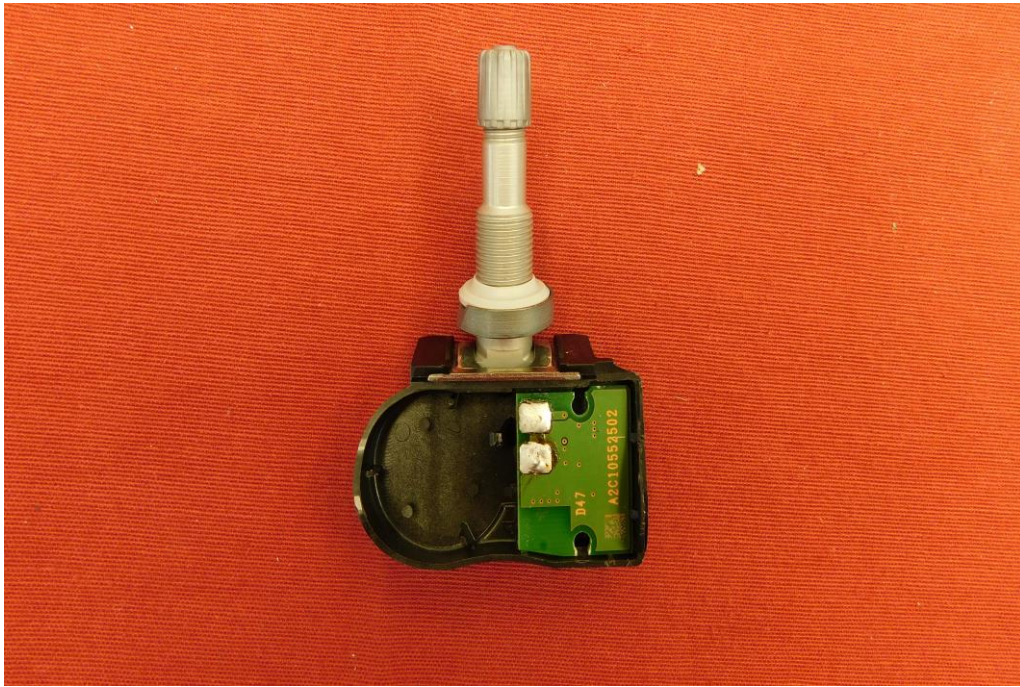
Picture 1: Opened TIS-15N, top view
