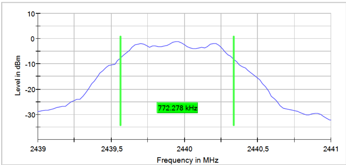
6 dB Bandwidth
