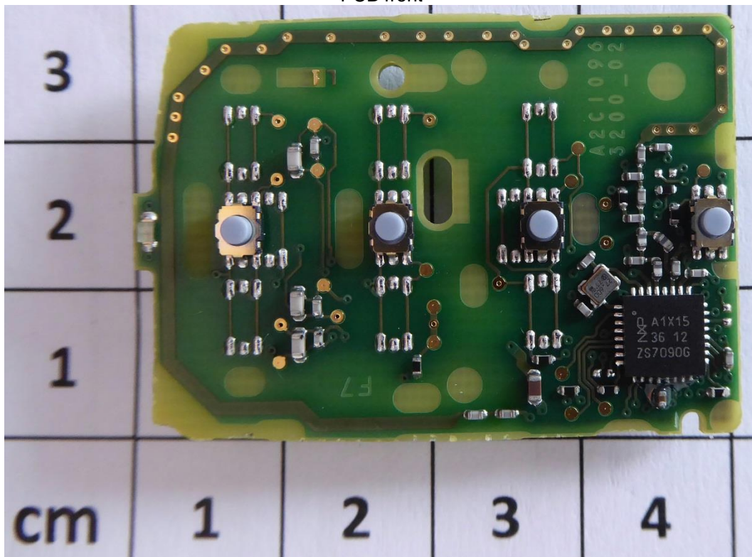
PCB front
