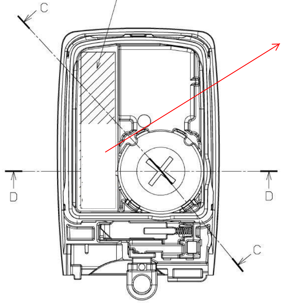
BACK VIEW (2:1) COVER REMOVED FOR CLARITY
