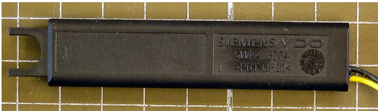
Antenna 5WK4 8774
