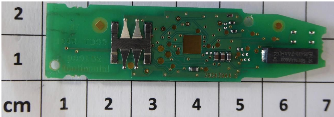
PCB front
