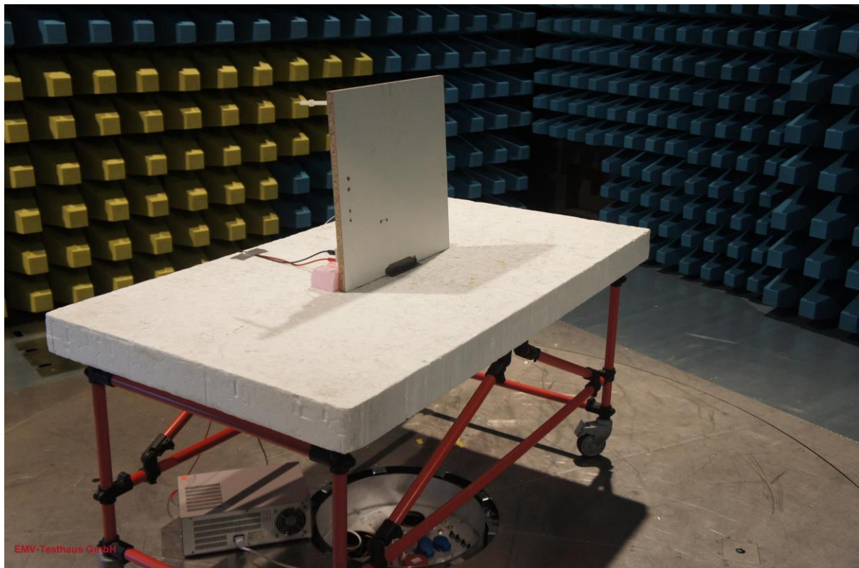
Picture 7: SAC, test setup radiated emission test above 1 GHz (rear view)
