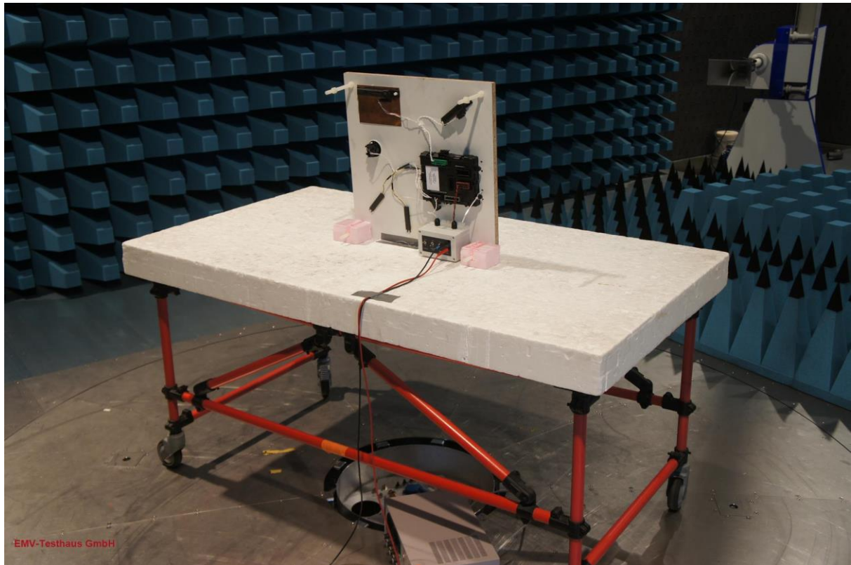
Picture 6: SAC, test setup radiated emission test above 1 GHz (front view)
