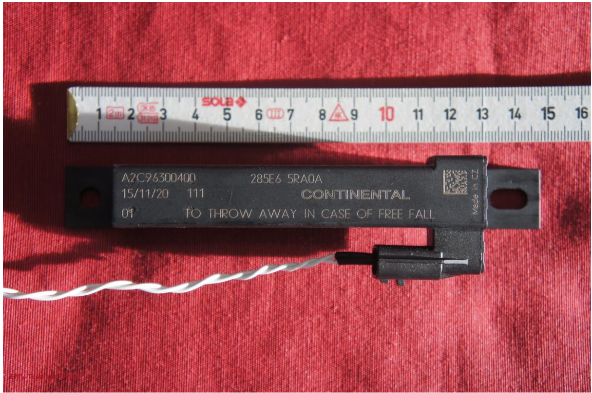
Picture 7: Middle antenna - front side
