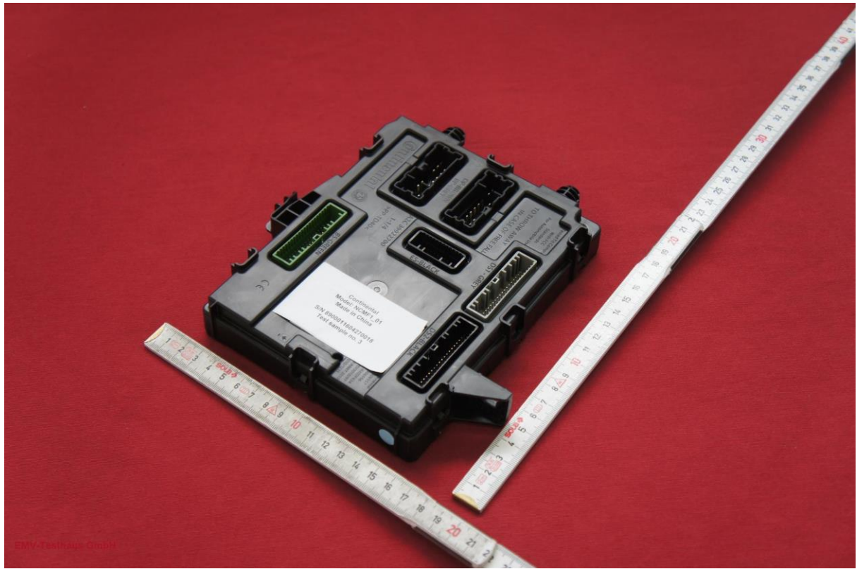
Picture 1: EUT - front view
