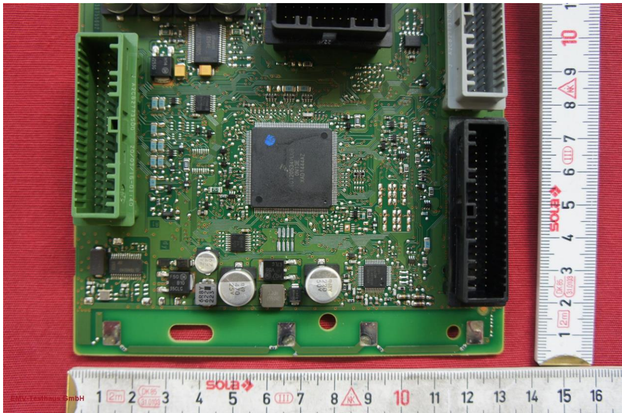
Picture 6: PCB - top side, detail lower half
