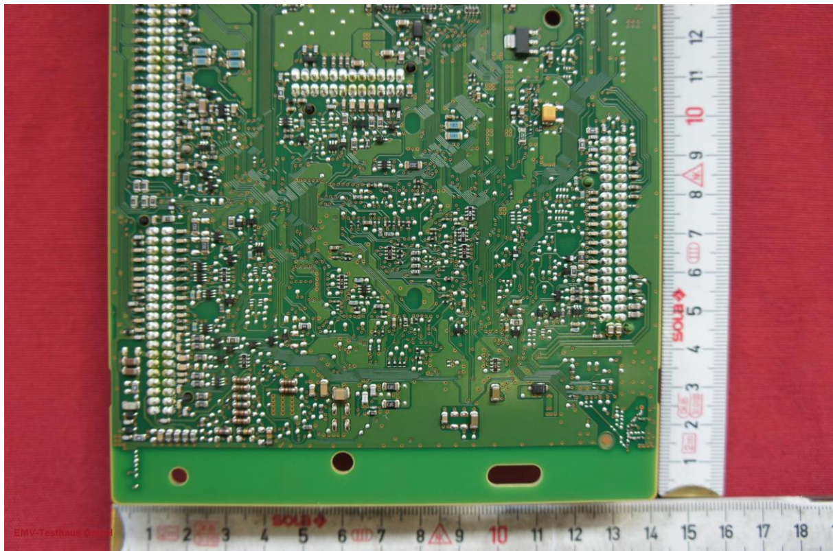
Picture 9: PCB - bottom side, detail lower half
