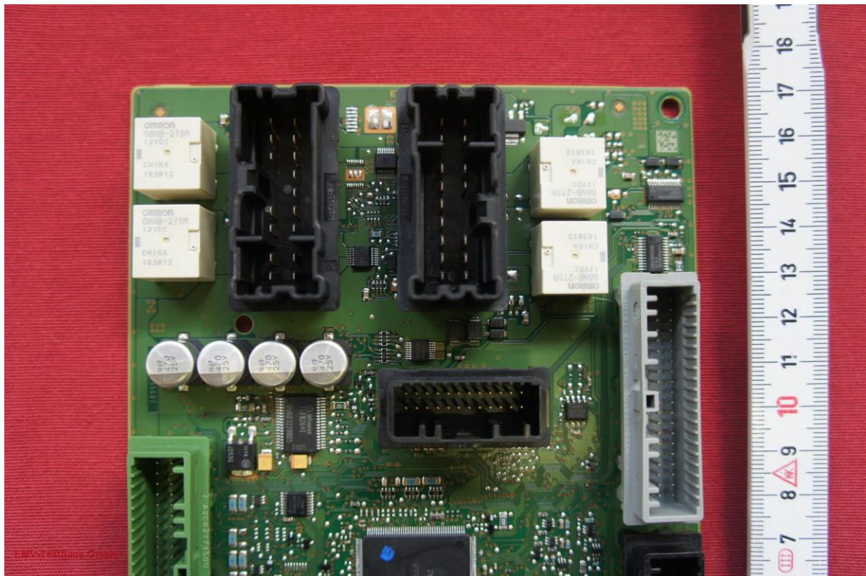
Picture 5: PCB - top side, detail upper half
