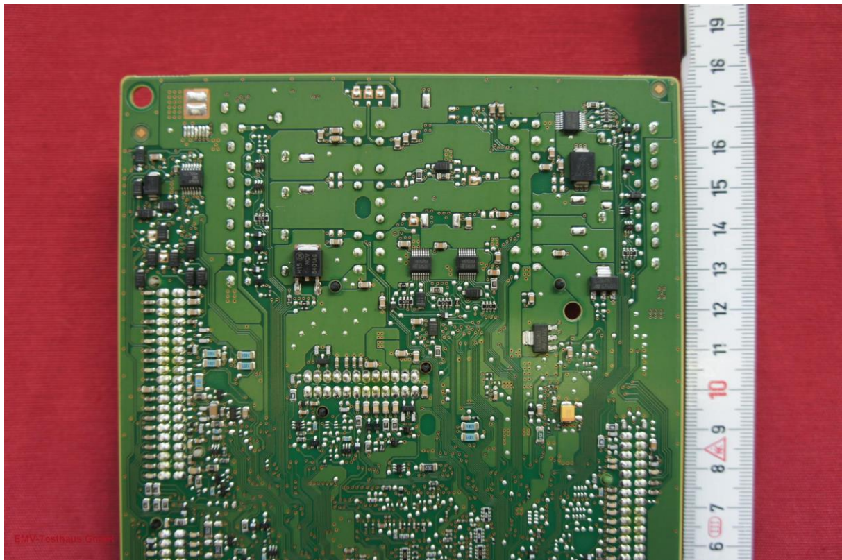
Picture 8: PCB - bottom side, detail upper half
