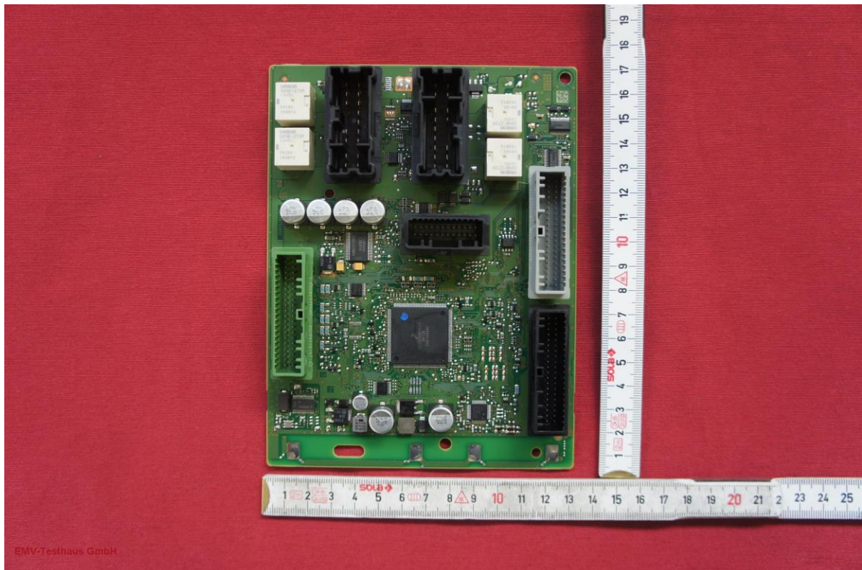
Picture 4: PCB - top side
