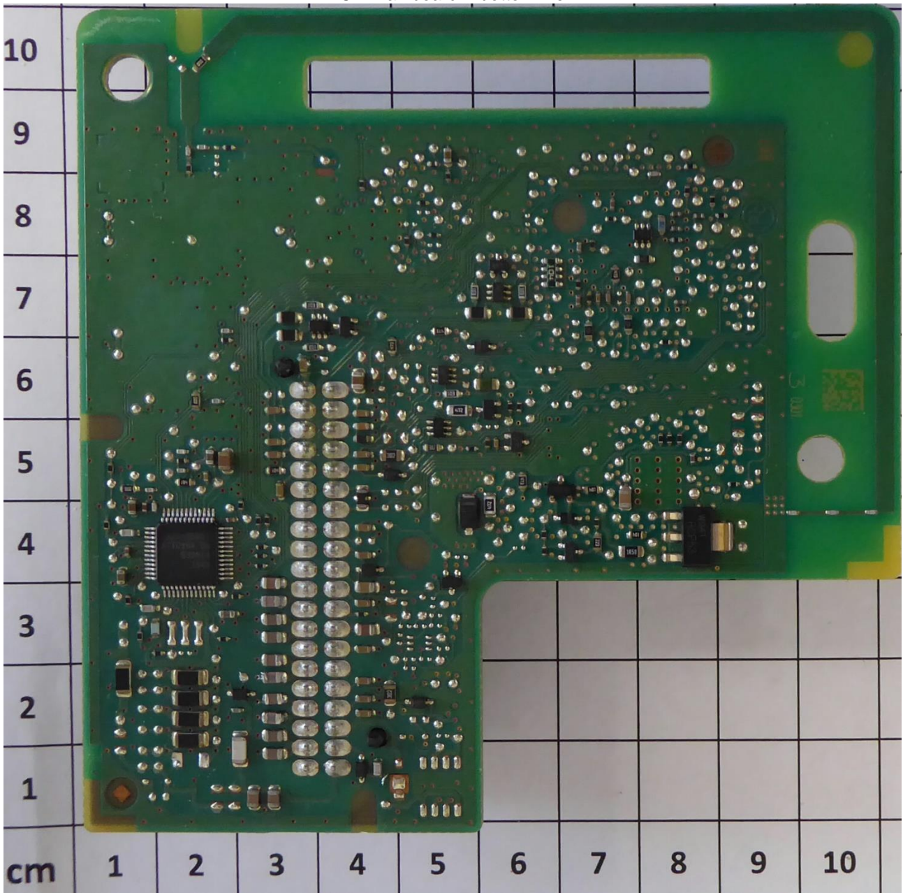
PCB mainboard – bottom view
