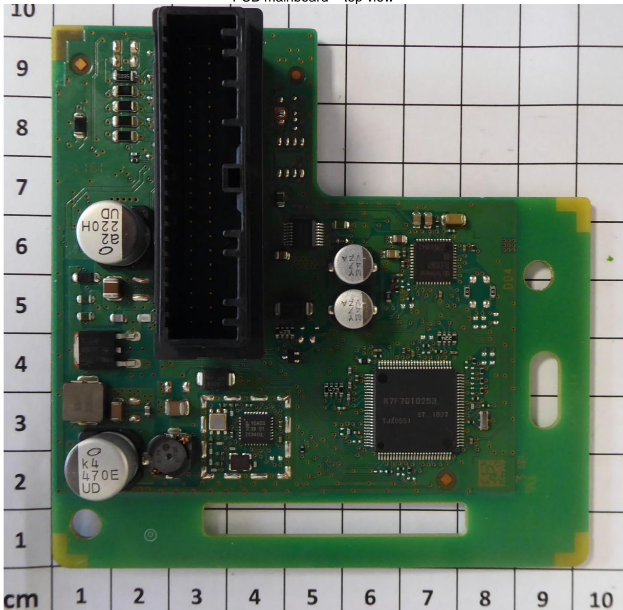
PCB mainboard – top view
