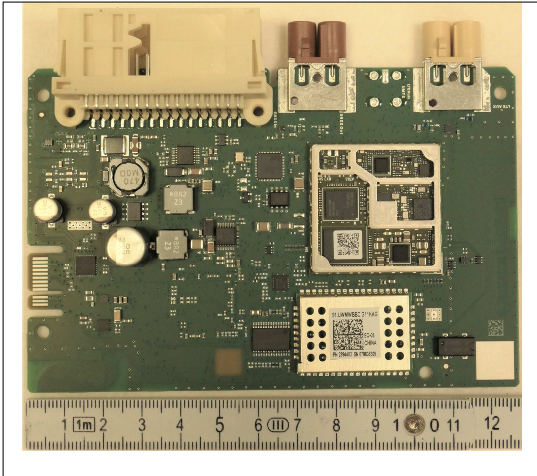
Figure9: PCB top view
