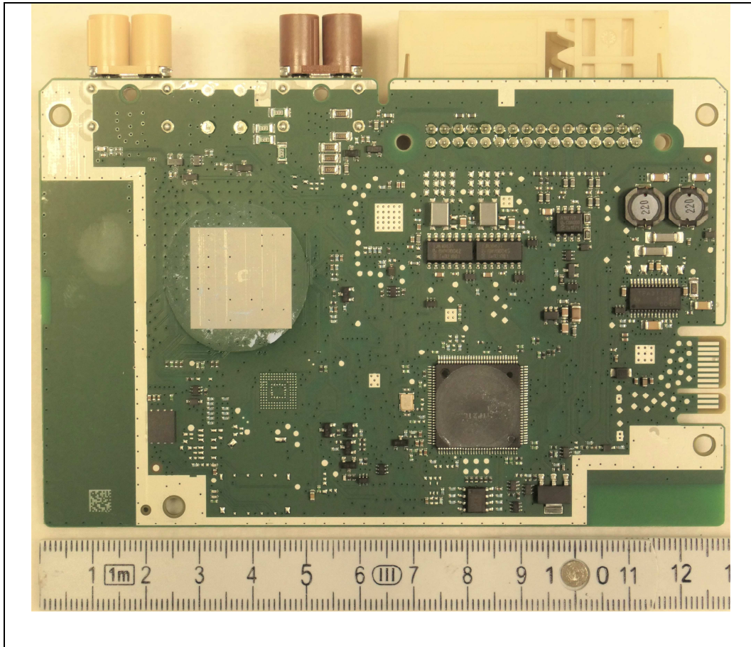
Figure8: PCB bottom view
