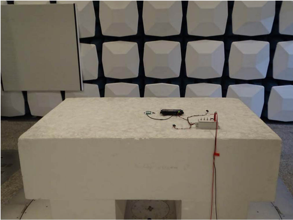
Back View of Radiated Test (External Antenna)
