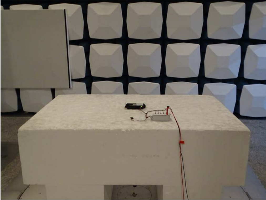
Back View of Radiated Test (Internal Antenna)
