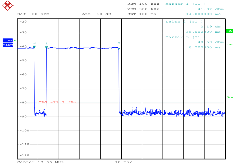
Plot 1: Timing of the Transmitter
