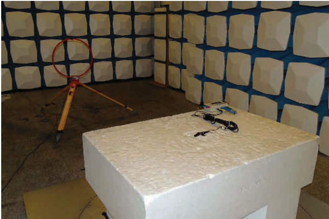
Back View of Radiated Test (Loop)
