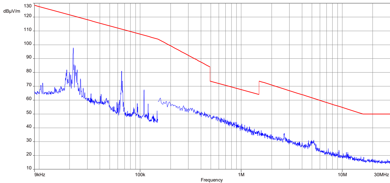
Plot 1: 9 kHz – 30 MHz, magnetic emissions, worst case
