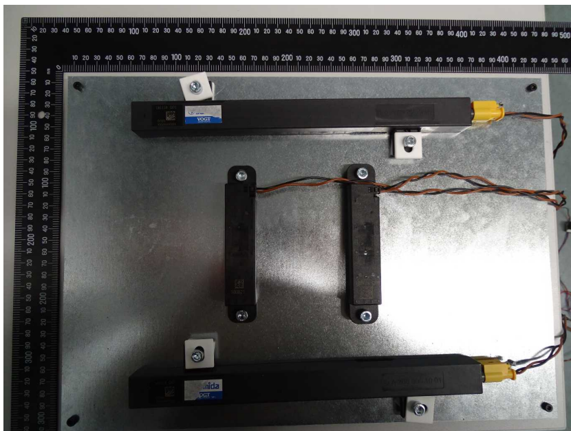
Photo 8: The four external antennas
