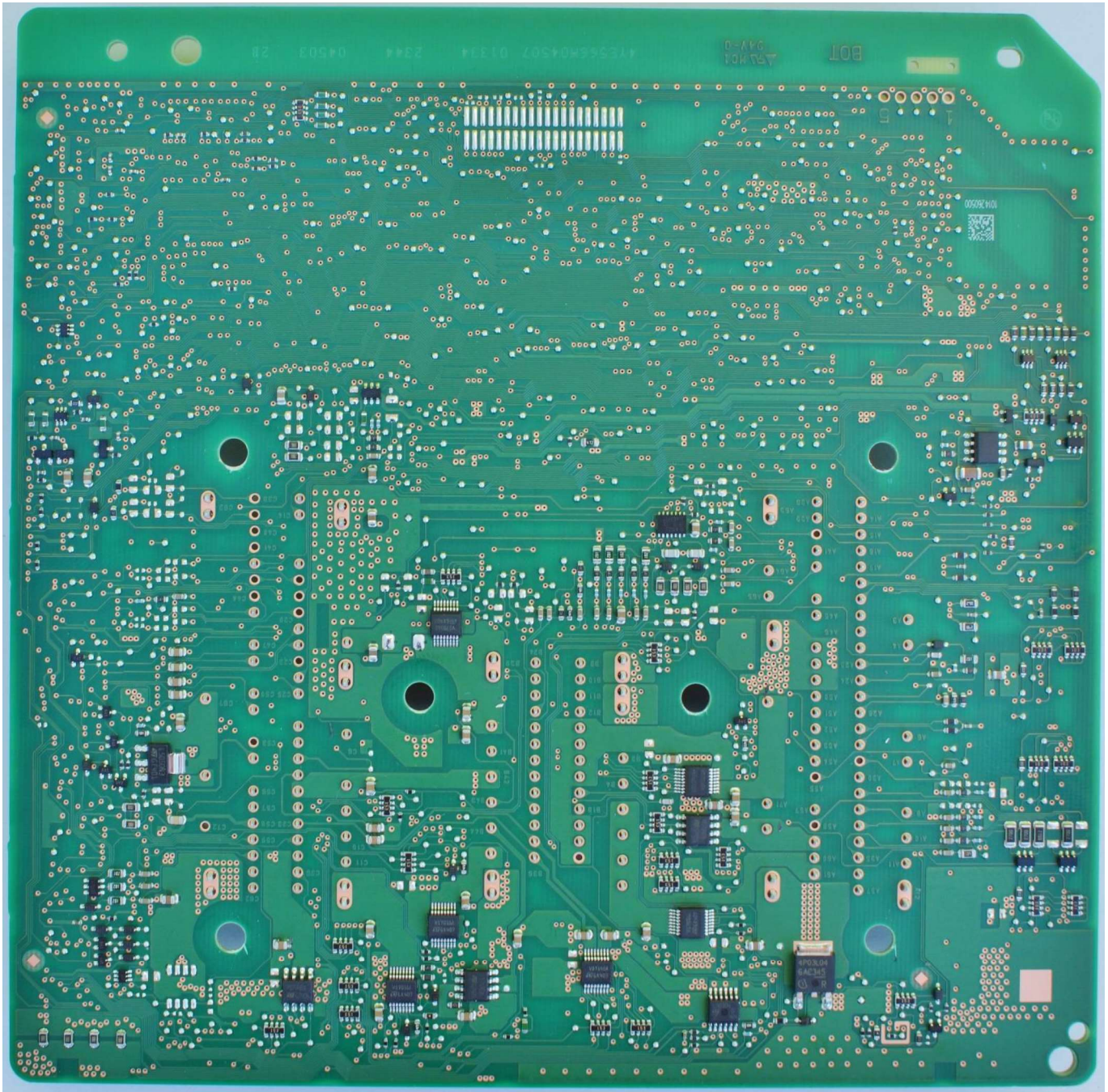
Bottom view of the Main-Board
