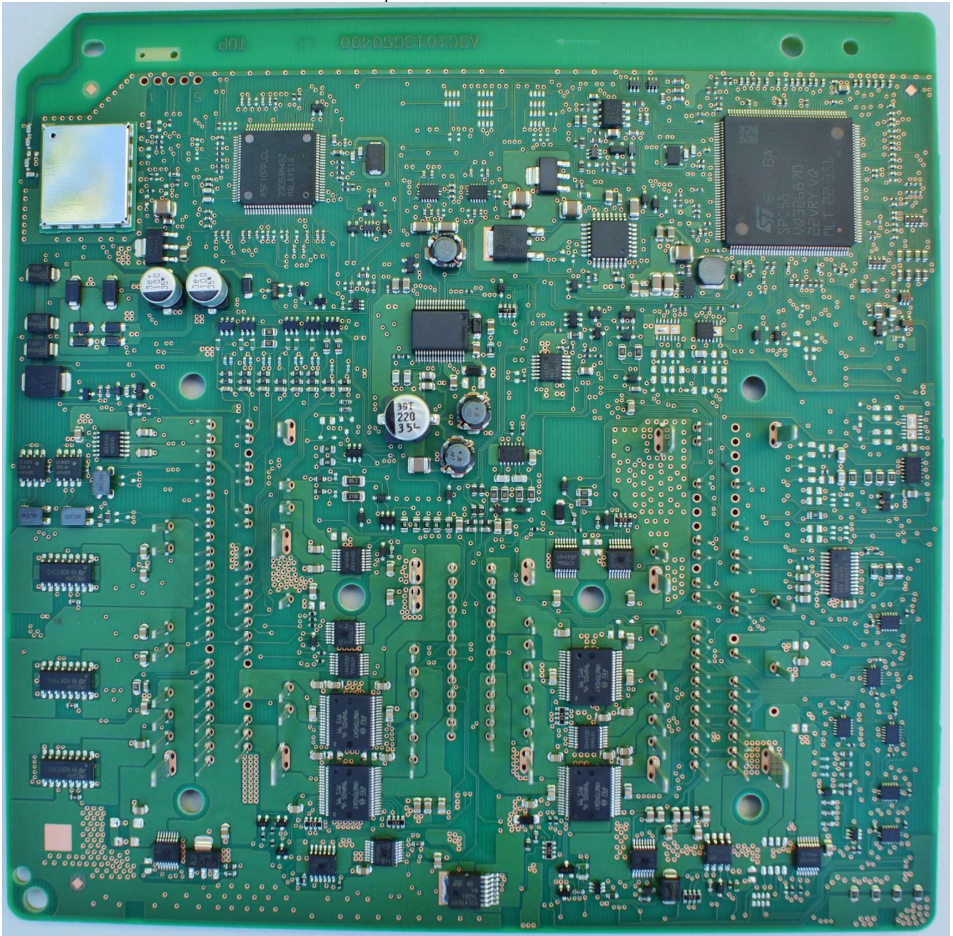
Top view of the Main-Board
