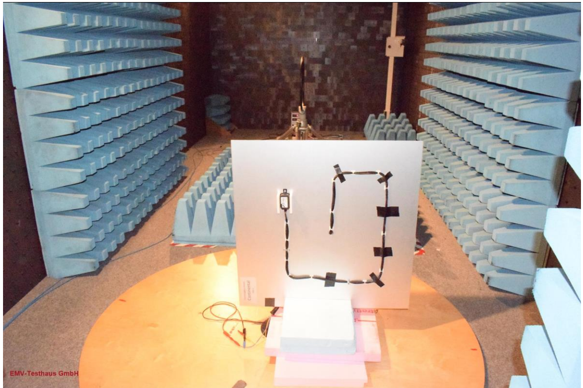
Picture 1: EUT test setup radiated emission test below 30 MHz
