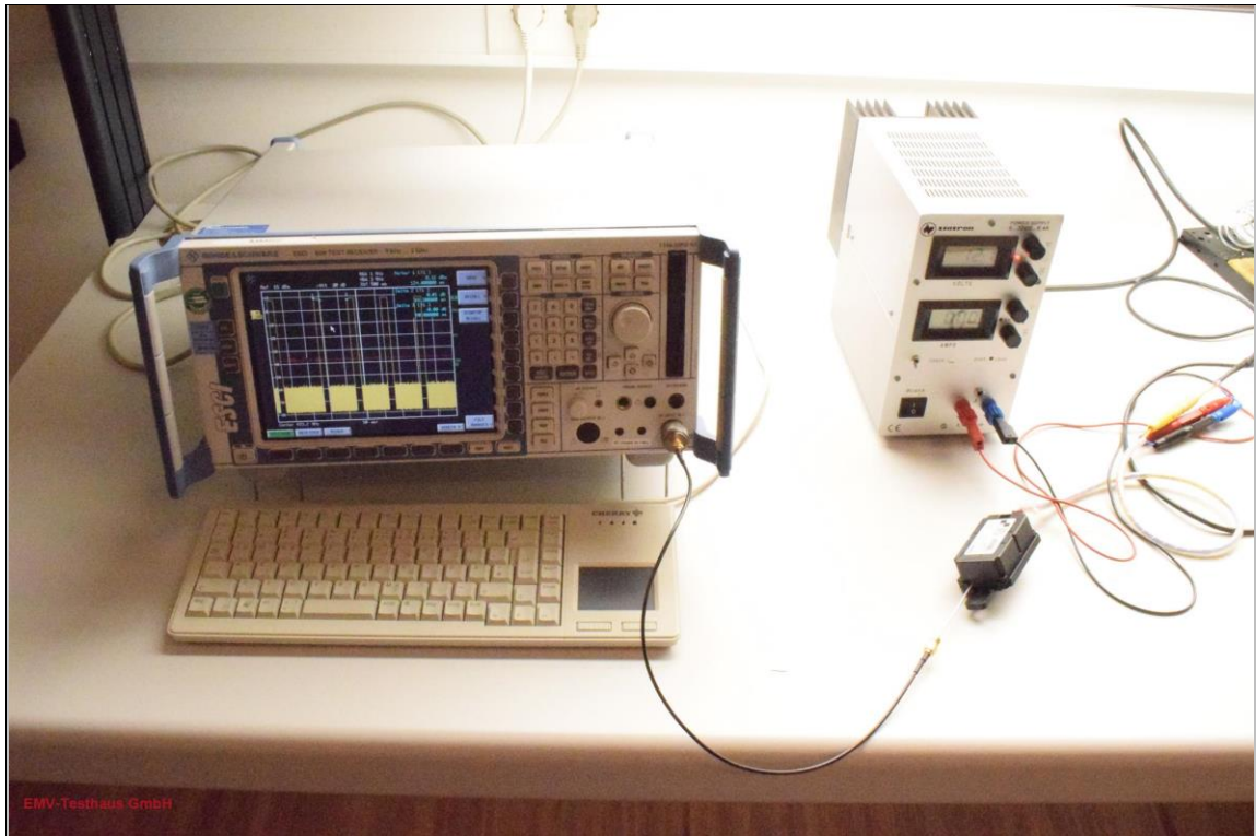
Picture 4: EUT test setup conducted measurements
