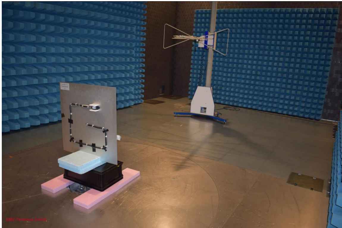
Picture 2: EUT test setup radiated emission test from 30 MHz to 1 GHz
