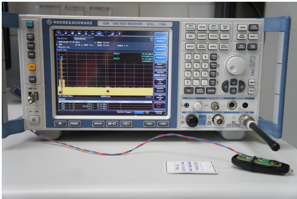
Picture 11: Relative measurement of signal deactivation
