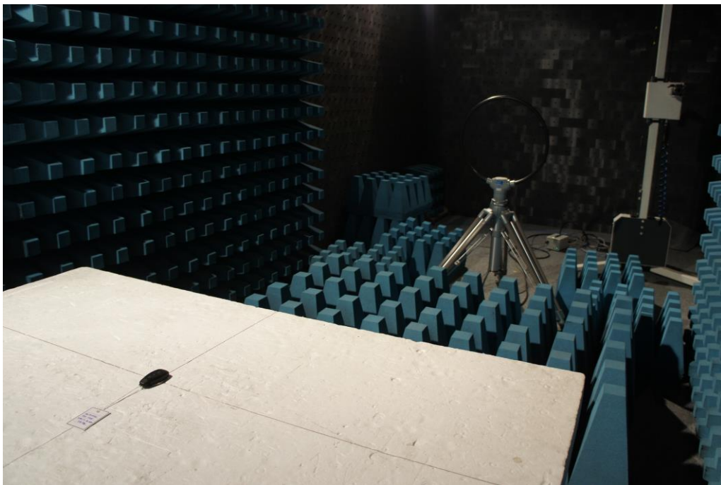
Picture 2: CDC, test setup radiated emission test 9 kHz -30 MHz (side view)
