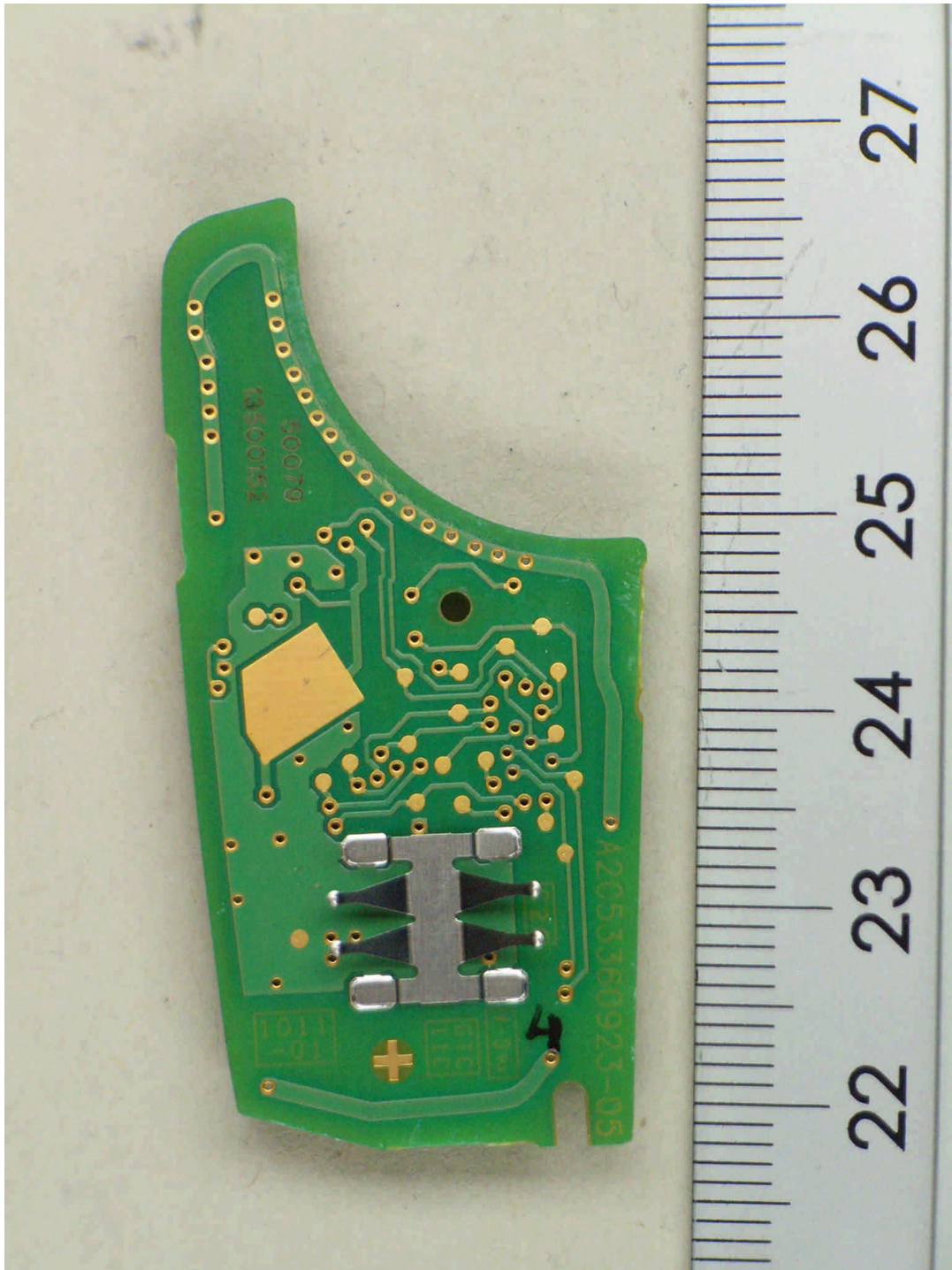
101794_22.jpg Global A Flap Key, PCB Matching N, bottom view
