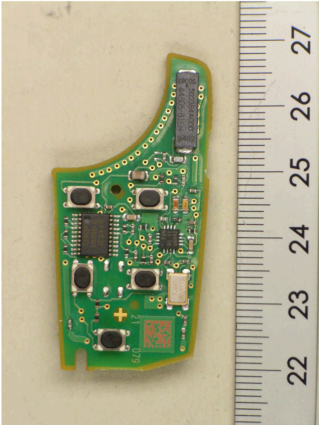
101794_21.jpg Global A Flap Key, PCB Matching N, top view
