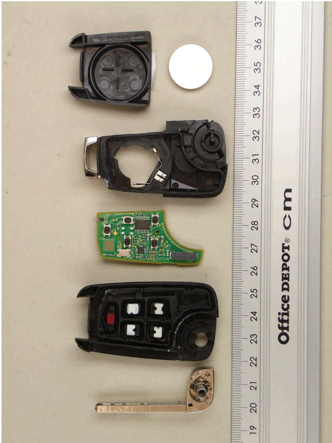
101794_20.jpg Global A Flap Key , internal view
