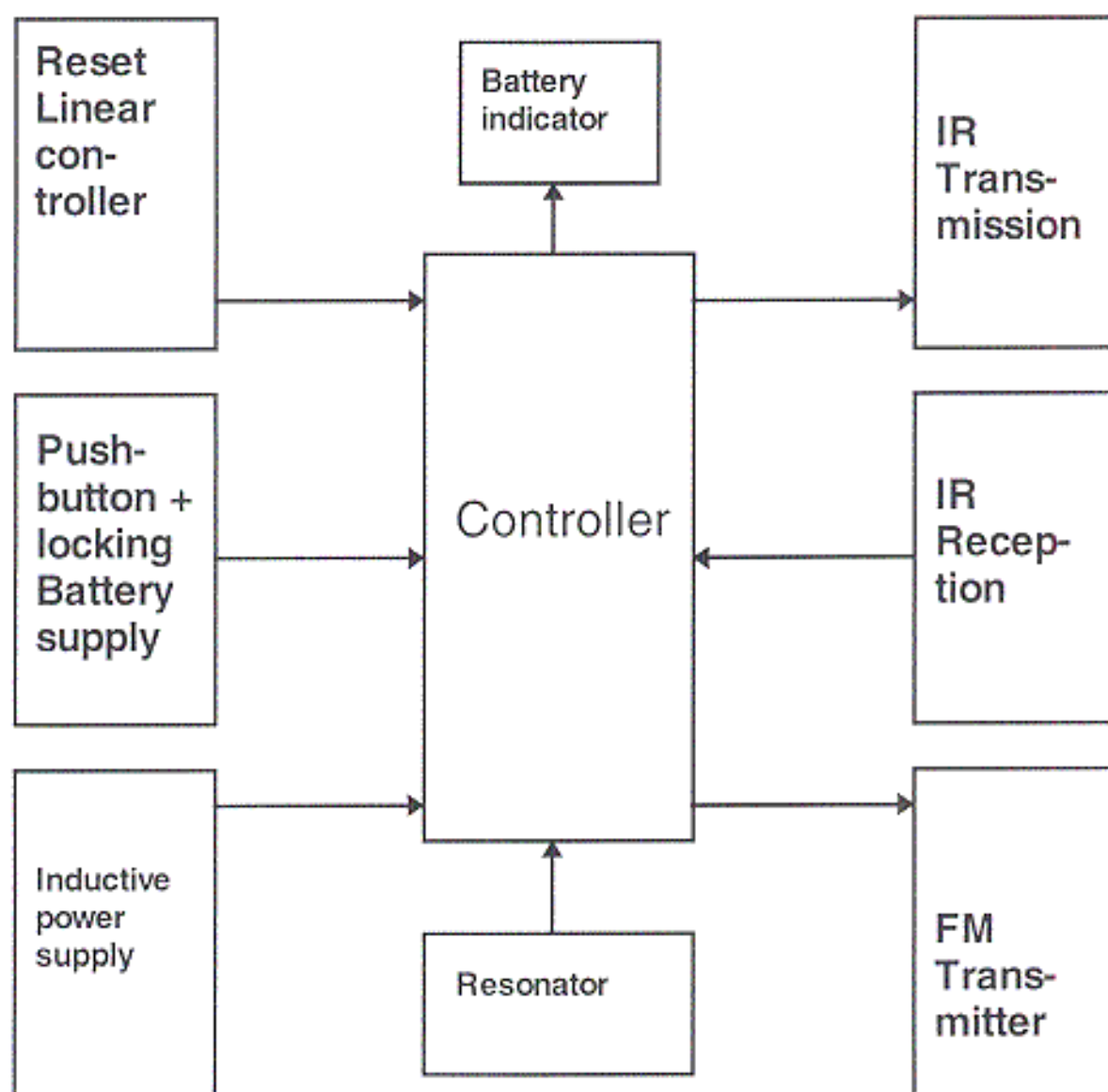
Fig. 2: Block diagram - Main key
