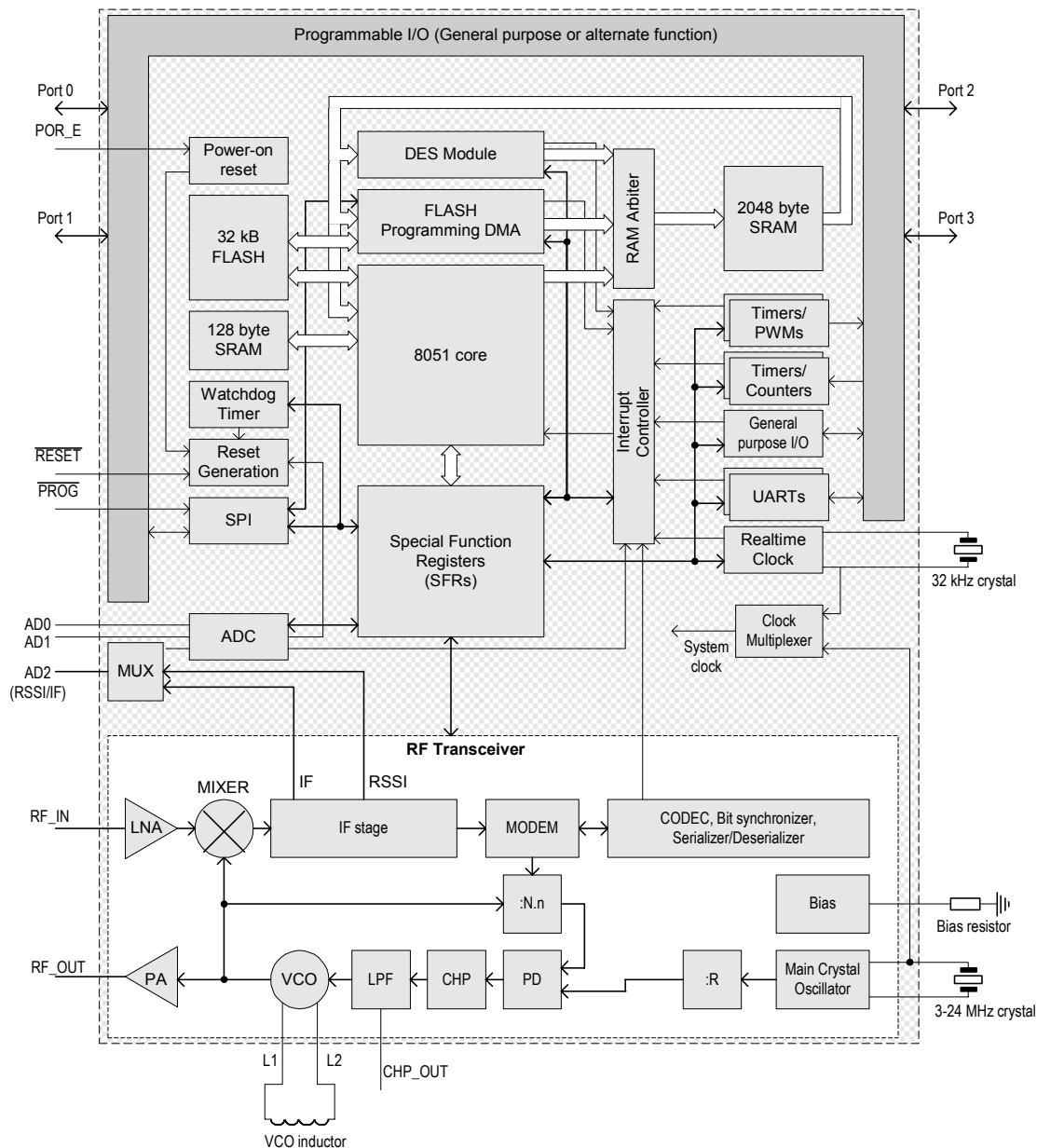
Figure 2. CC1010 Block Diagram
