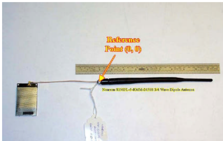
< Nearson, S191FL-5-RMM-2450S ¾ wave dipole antenna with 10mW unit >
