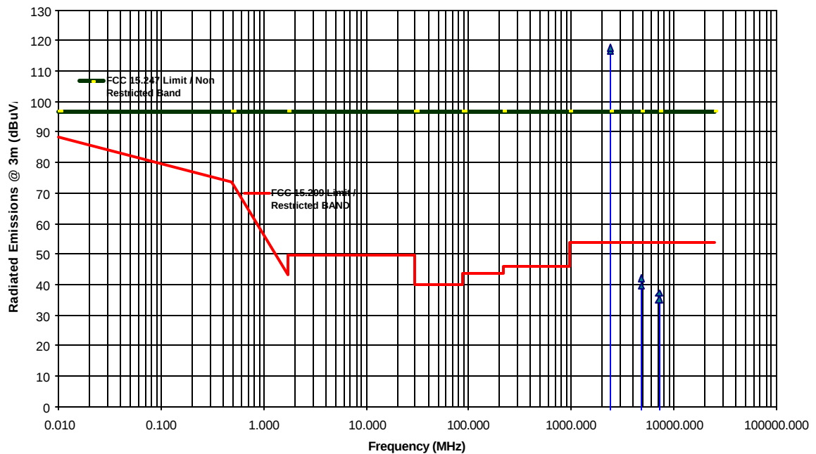
Transmitter Radiated Emissions Measurements at 3 Meter OFTS Aerocomm LX2400-150 FHSS 148 mW Transmitter Tx Freq.: 2402 MHz, Antenna: Nearson S191FL-RMM-2450S
