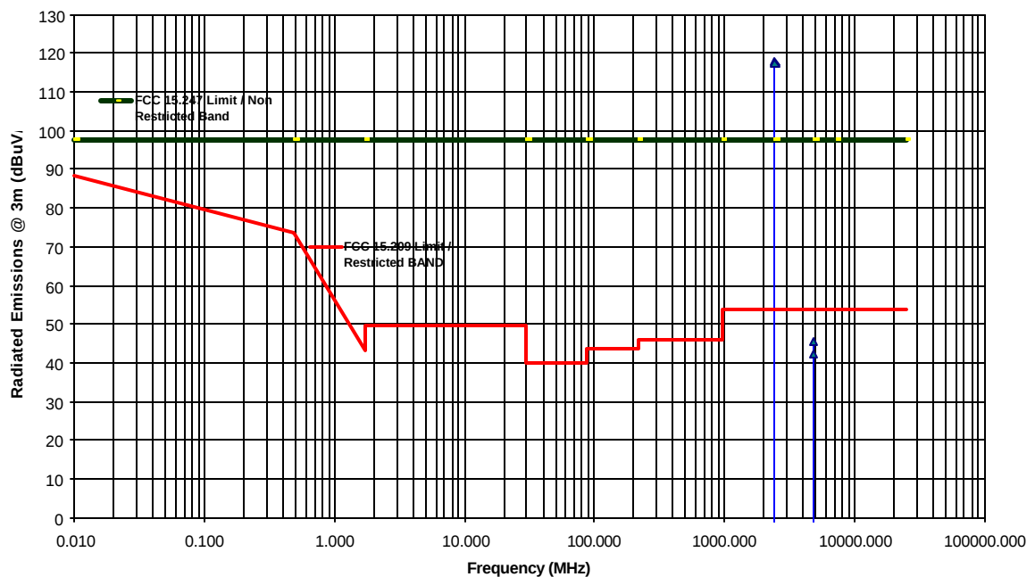
Transmitter Radiated Emissions Measurements at 3 Meter OFTS Aerocomm LX2400-150 FHSS 148 mW Transmitter Tx Freq.:2440 MHz, Antenna: Nearson S131CL-RMM-2450S
