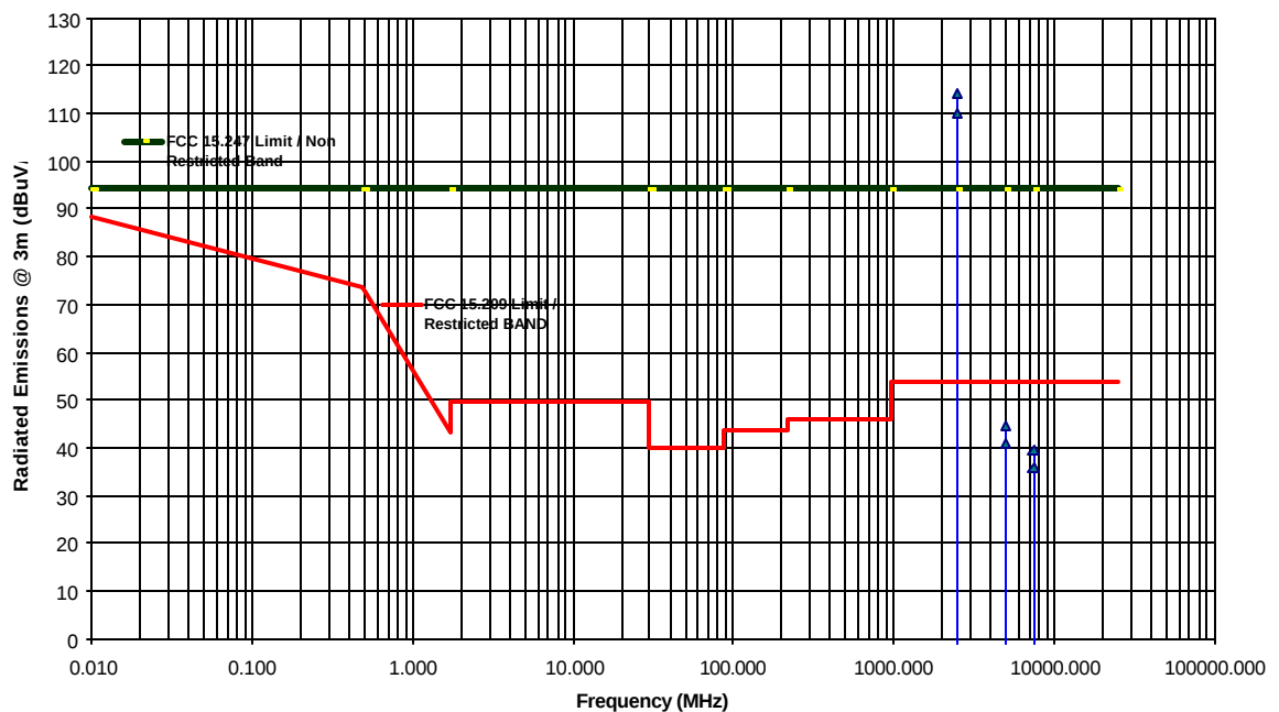
Transmitter Radiated Emissions Measurements at 3 Meter OFTS Aerocomm LX2400-150 FHSS 148 mW Transmitter Tx Freq.:2478 MHz, Antenna: Aerocomm NZH2400-MMCX Antenna
