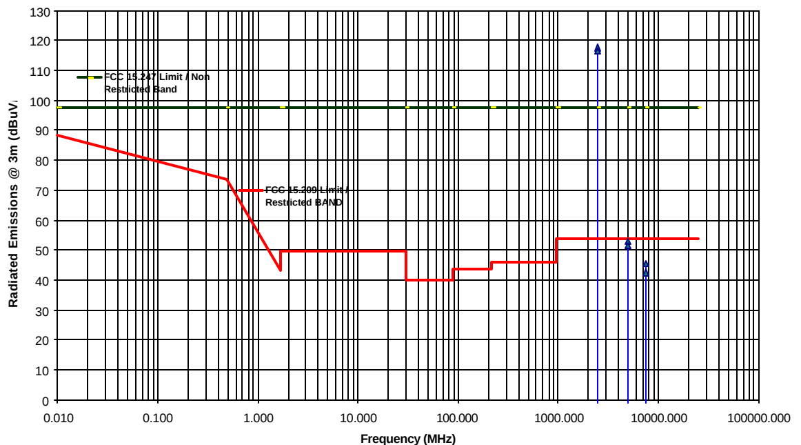
Transmitter Radiated Emissions Measurements at 3 Meter OETS Aerocomm LX2400-150 FHSS 148 mW Transmitter Tx Freq.:2478 MHz, Antenna: Nearson S131CL-RMM-2450S
