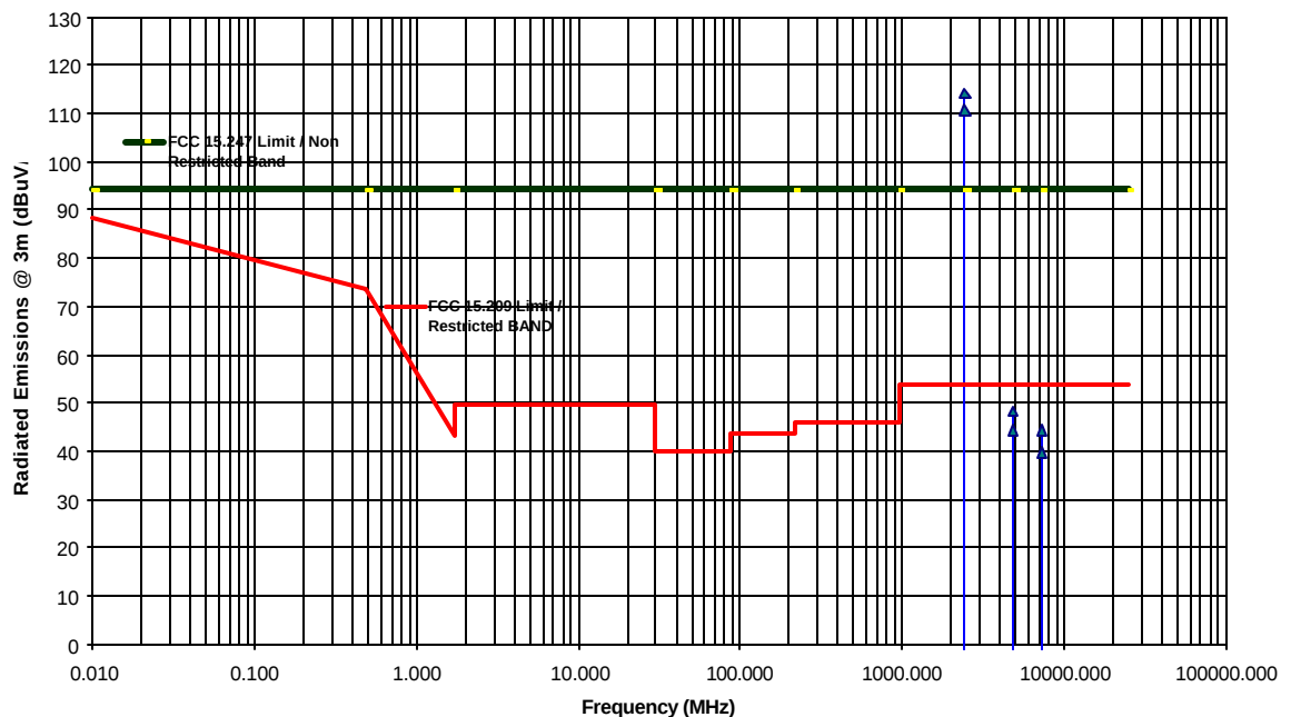
Transmitter Radiated Emissions Measurements at 3 Meter OFTS Aerocomm LX2400-150 FHSS 148 mW Transmitter Tx Freq.:2440 MHz, Antenna: Aerocomm NZH2400-MMCX Antenna
