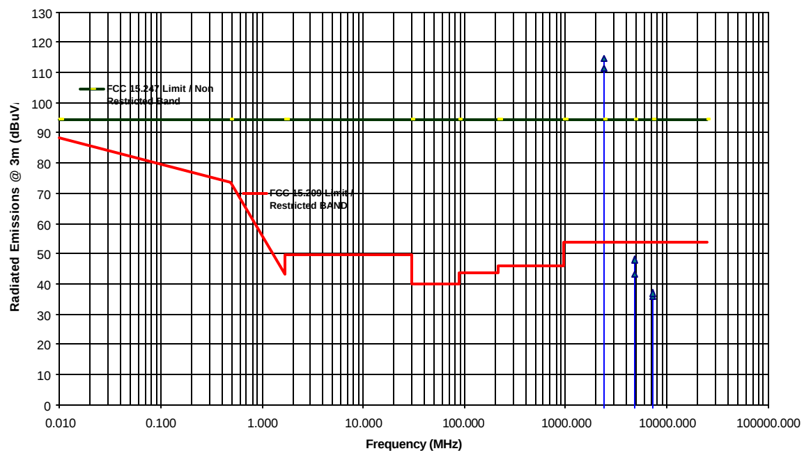
Transmitter Radiated Emissions Measurements at 3 Meter OFTS Aerocomm LX2400-150 FHSS 148 mW Transmitter Tx Freq.:2402 MHz, Antenna: Aerocomm NZH2400-MMCX Antenna
