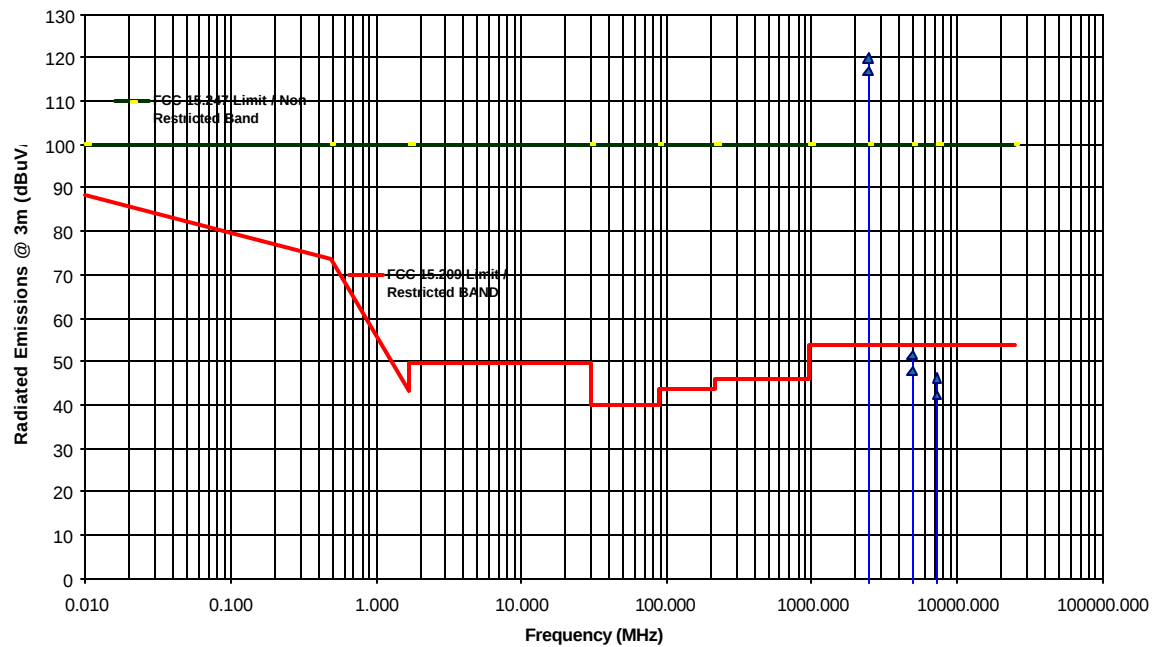
Transmitter Radiated Emissions Measurements at 3 Meter OFTS Aerocomm LX2400-150 FHSS 148 mW Transmitter Tx Freq.:2440 MHz, Antenna: Maxrad MC2400 Antenna
