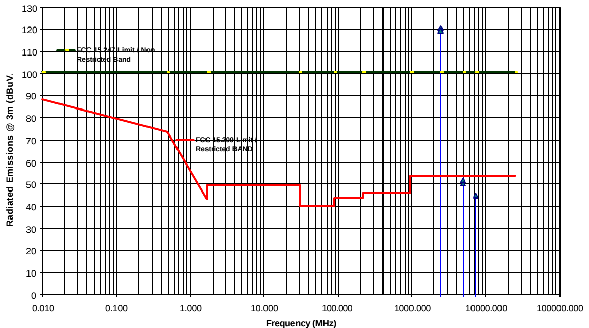
Transmitter Radiated Emissions Measurements at 3 Meter OFTS Aerocomm LX2400-150 FHSS 148 mW Transmitter Tx Freq.: 2440 MHz, Antenna: Nearson S181FL-RMM-2450S
