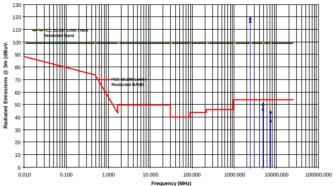
Transmitter Radiated Emissions Measurements at 3 Meter OFTS Aerocomm LX2400-150 FHSS 148 mW Transmitter Tx Freq.:2402 MHz, Antenna: Centurion WCP2400-MMCX
