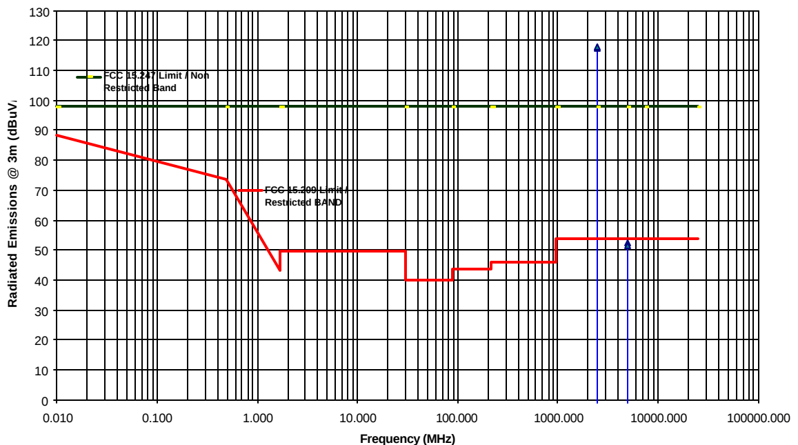
Transmitter Radiated Emissions Measurements at 3 Meter OFTS Aerocomm LX2400-150 FHSS 148 mW Transmitter Tx Freq.: 2478 MHz, Antenna: Nearson S191FL-RMM-2450S
