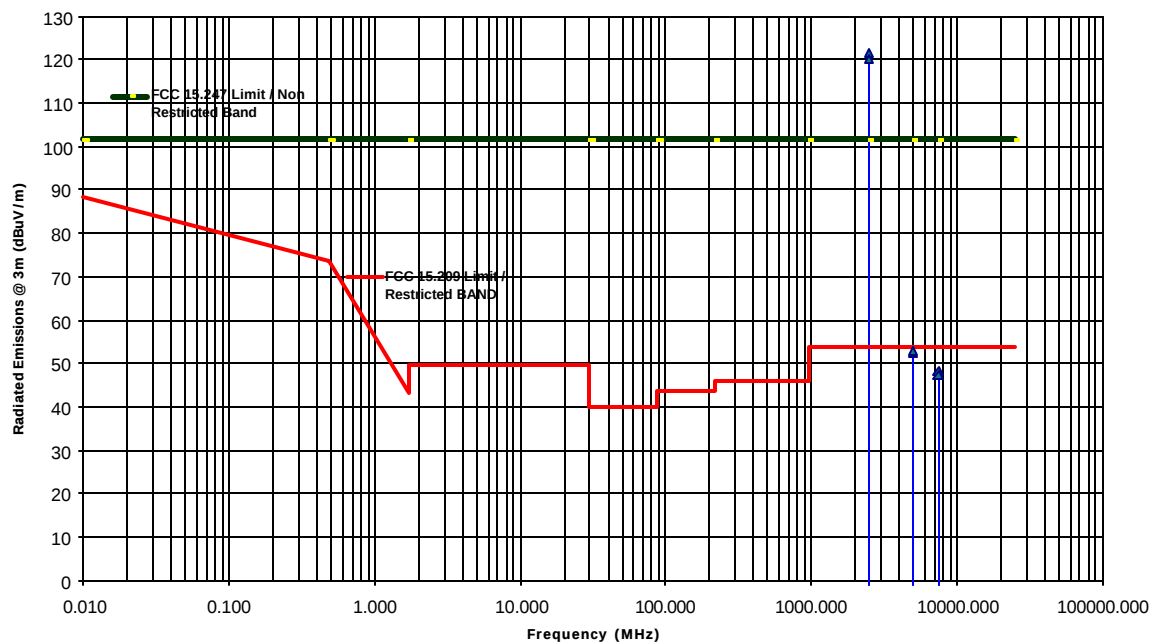
Transmitter Radiated Emissions Measurements at 3 Meter OFTS Aerocomm LX2400-150 FHSS 148 mW Transmitter Tx Freq.: 2478 MHz, Antenna: Nearson S181FL-RMM-2450S
