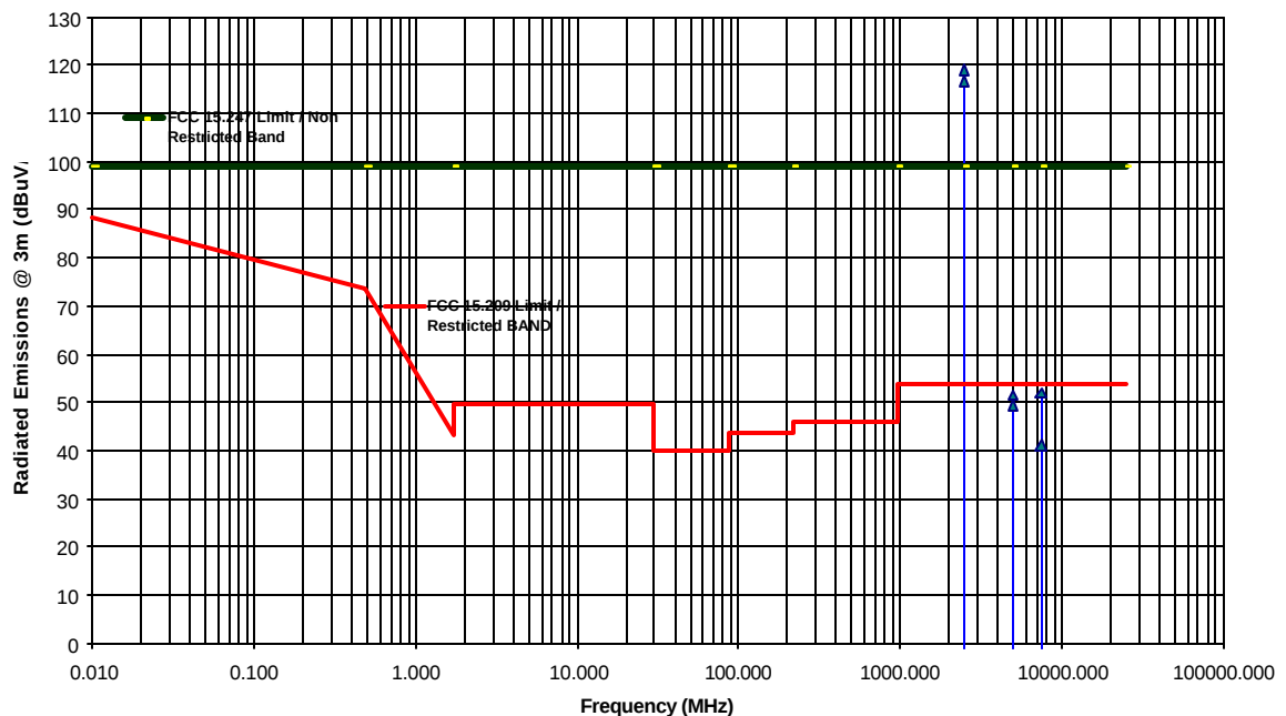
Transmitter Radiated Emissions Measurements at 3 Meter OFTS Aerocomm LX2400-150 FHSS 148 mW Transmitter Tx Freq.:2478 MHz, Antenna: Maxrad MC2400 Antenna
