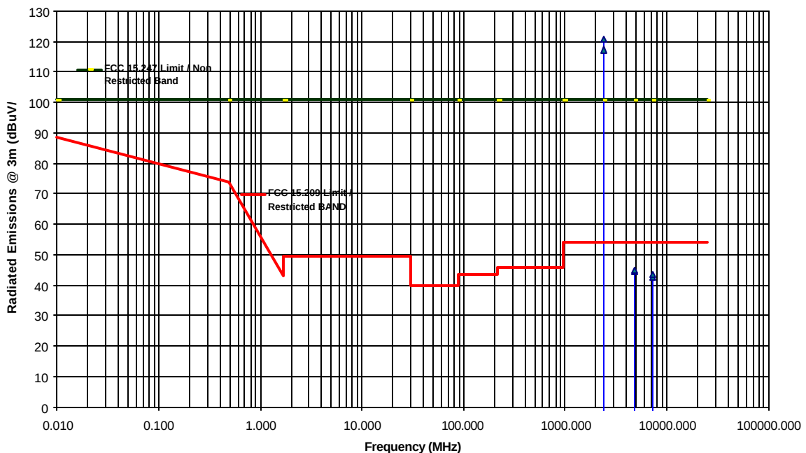
Transmitter Radiated Emissions Measurements at 3 Meter OETS Aerocomm LX2400-150 FHSS 148 mW Transmitter Tx Freq.:2402 MHz, Antenna: Maxrad MC2400 Antenna
