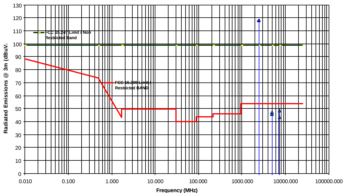
Transmitter Radiated Emissions Measurements at 3 Meter OFTS Aerocomm LX2400-150 FHSS 148 mW Transmitter Tx Freq.: 2440 MHz, Antenna: Nearson S191FL-RMM-2450S
