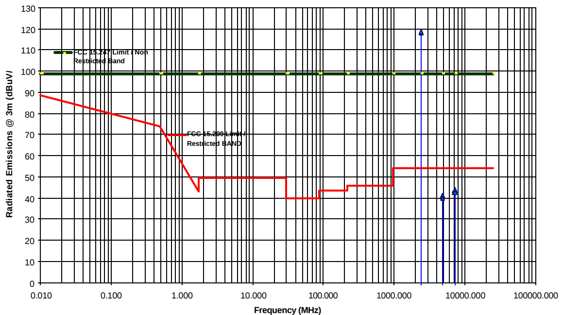
Transmitter Radiated Emissions Measurements at 3 Meter OFTS Aerocomm LX2400-150 FHSS 148 mW Transmitter Tx Freq.: 2402 MHz, Antenna: Nearson S181FL-RMM-2450S
