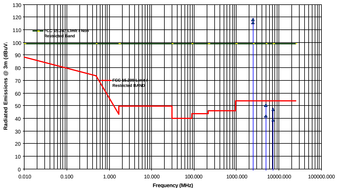
Transmitter Radiated Emissions Measurements at 3 Meter OFTS Aerocomm LX2400-150 FHSS 148 mW Transmitter Tx Freq.:2440 MHz, Antenna: Centurion WCP2400-MMCX
