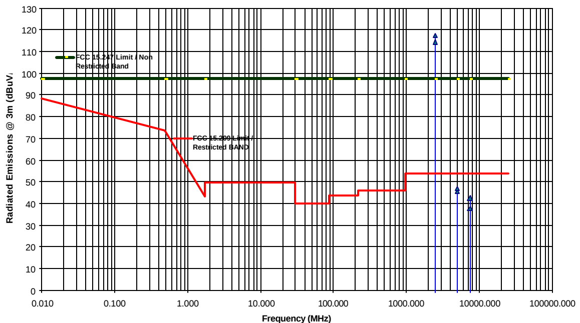
Transmitter Radiated Emissions Measurements at 3 Meter OFTS Aerocomm LX2400-150 FHSS 148 mW Transmitter Tx Freq.:2478 MHz, Antenna: Centurion WCP2400-MMCX
