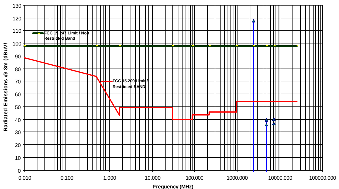
Transmitter Radiated Emissions Measurements at 3 Meter OFTS Aerocomm LX2400-150 FHSS 148 mW Transmitter Tx Freq.:2402 MHz, Antenna: Nearson S131CL-RMM-2450S
